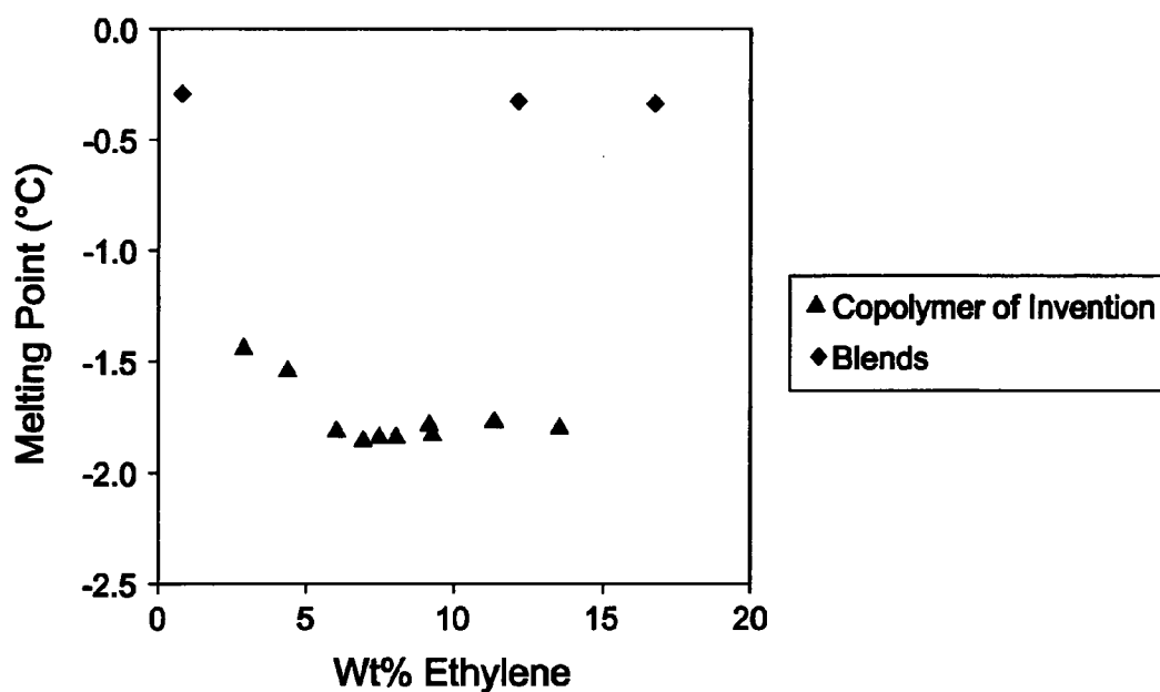
Fig. 4 Variation of Melting Point by DSC with composition (Wt% Ethylene)
