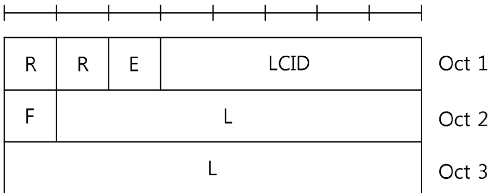
R/R/E/LCID/F/L sub-header with 15-bit L field
