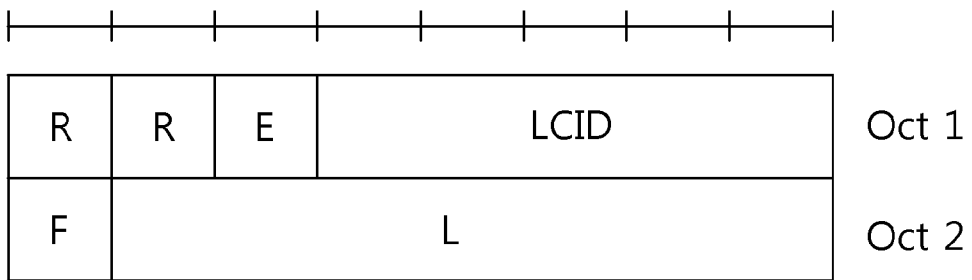
R/R/E/LCID/F/L sub-header with 7-bit L field
