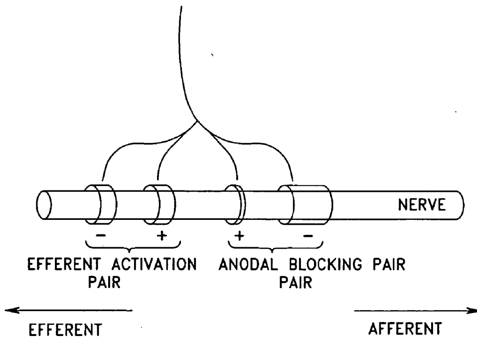
FIGURE Y-QUADRAPOLAR BLOCKING ELECTRODE
