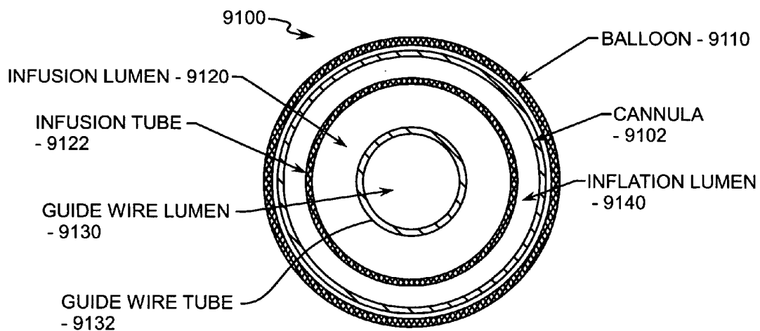
CROSS-SECTIONAL VIEW A-A
