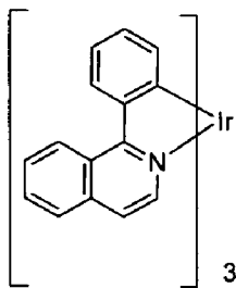
Ir(1-piq) 3
