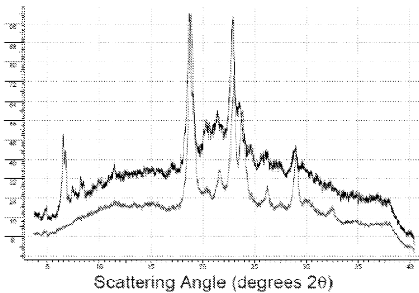
XRPD pattern obtained for "Form U 20 pass" lyophilic sample (black trace) and XRPD pattern of CoQ10 bulk drug substance (red trace). The pattern has been normalized so that the intensity of the most intense peak equals 100%.
