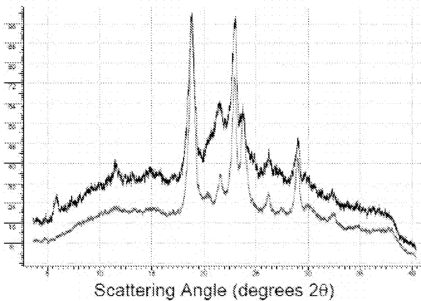
XRPD pattern obtained for "Form G 20 pass" lyophilic sample (black trace) and XRPD pattern of CoQ10 bulk drug substance (red trace). The pattern has been normalized so that the intensity of the most intense peak equals 100%.
