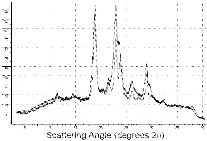
XRPD pattern obtained for "Form T 20 pass" lyophilic sample (black trace) and XRPD pattern of CoQ10 bulk drug substance (red trace). The pattern has been normalized so that the intensity of the most intense peak equals 100%.
