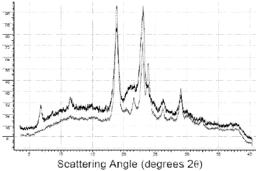
XRPD pattern obtained for "Form Q 20 pass" lyophilic sample (black trace) and XRPD pattern of CoQ10 bulk drug substance (red trace). The pattern has been normalized so that the intensity of the most intense peak equals 100%.
