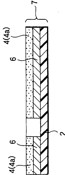
FIG.1C ETCHING PROCESS
