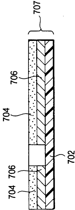
FIG.11C ETCHING PROCESS
