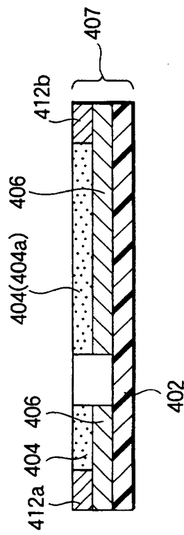
FIG.8C ETCHING PROCESS
