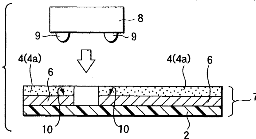
FIG.1D ULTRASONIC MOUNTING PROCESS
