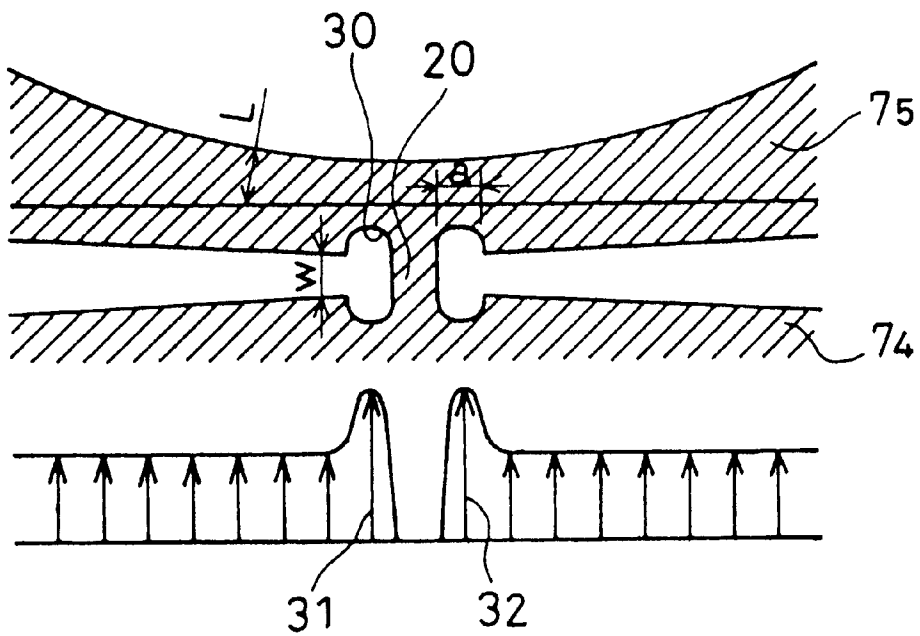
Fig. 24b PRIOR ART
