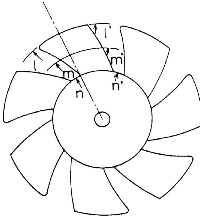
Fig.17a PRIOR ART
