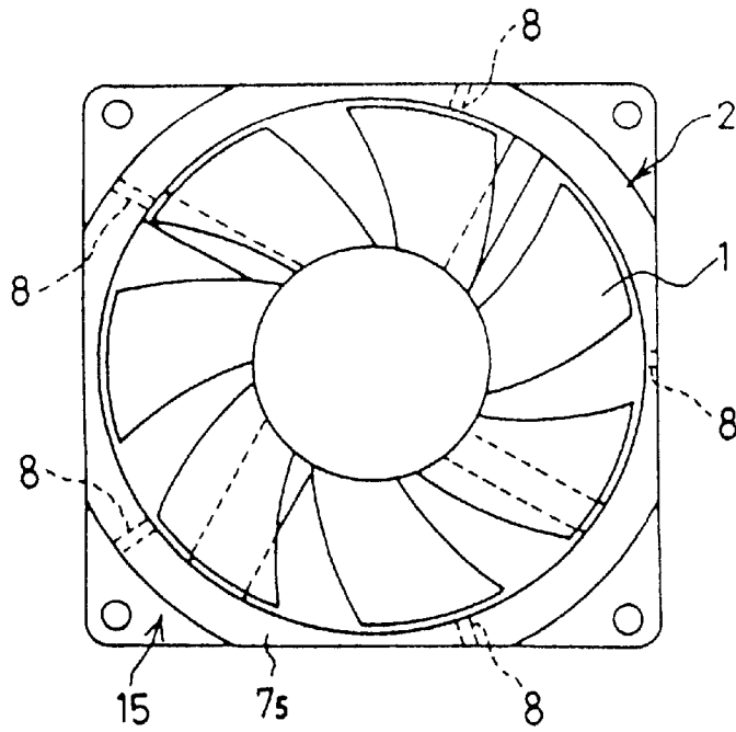
Fig.13a PRIOR ART
