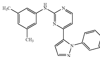
1-9 N-(3,5-dimethylphenyl)-4-(1-phenyl-1H-pyrazol-5-yl)pyrimidin-2-amine
