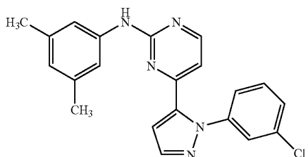
4-[1-(3-chlorophenyl)-1H-pyrazol-5-yl]-N-(3,5-dimethylphenyl)pyrimidin-2-amine;
