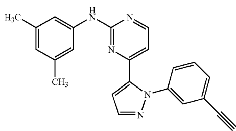
N-(3,5-dimethylphenyl)-4-[1-(3-ethynylphenyl)-1H-pyrazol-5-yl]pyrimidin-2-amine;
