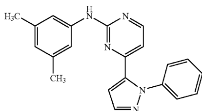
N-(3,5-dimethylphenyl)-4-(1-phenyl-1H-pyrazol-5-yl)pyrimidin-2-amine;
