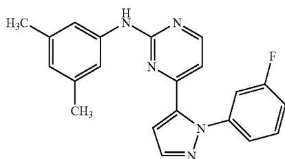
N-(3,5-dimethylphenyl)-4-[1-(3-fluorophenyl)-1H-pyrazol-5-yl]pyrimidin-2-amine;
