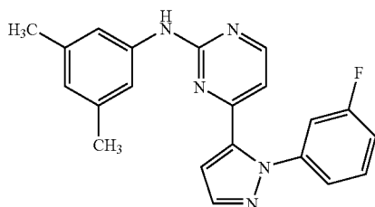
N-(3,5-dimethylphenyl)-4-[1-(3-fluorophenyl)-1H-pyrazol-5-yl]pyrimidin-2-amine
