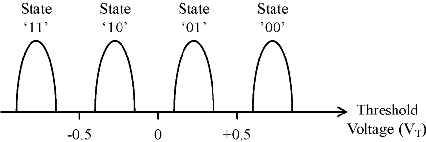
Multi-Level Cell
