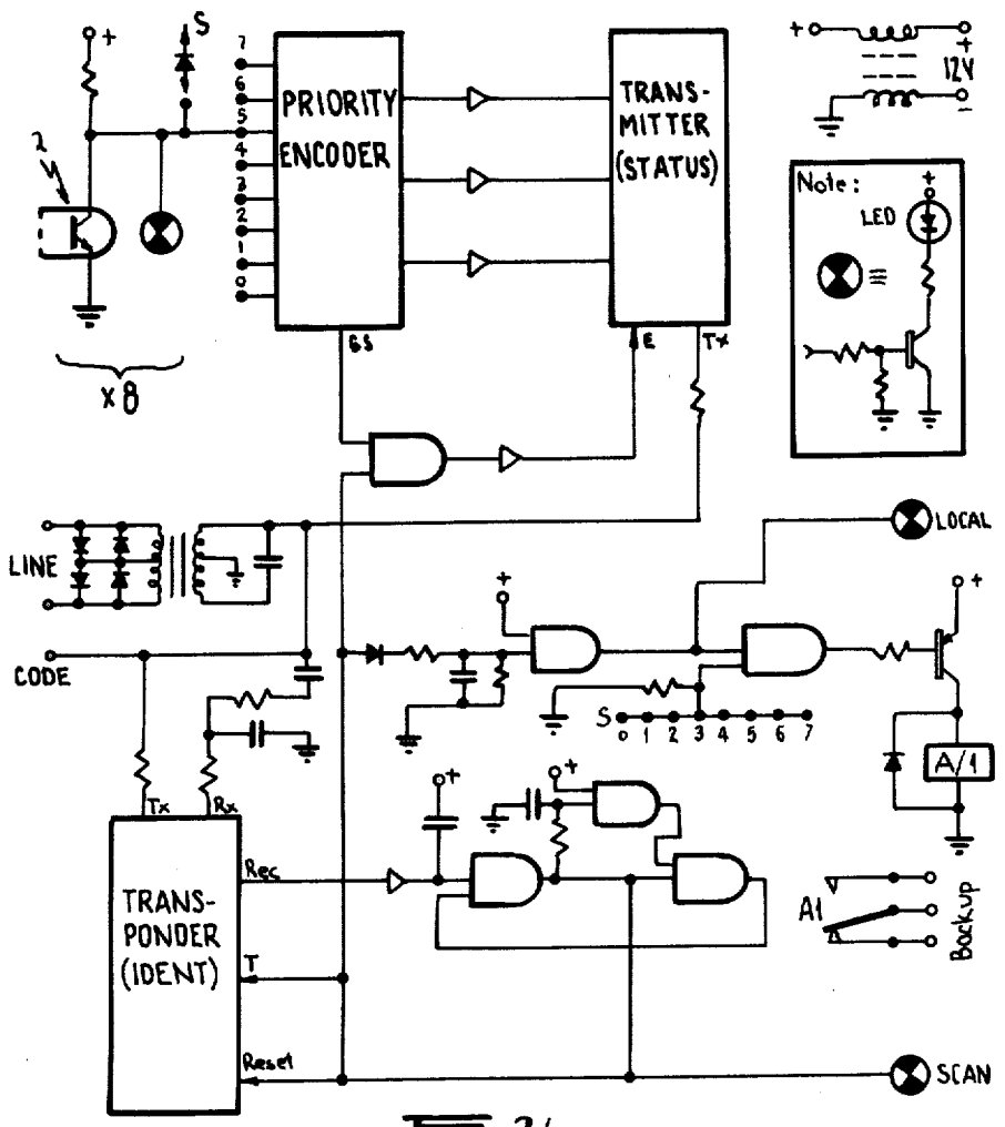
FIG. 3b. LINE CIRCUIT SECTION
