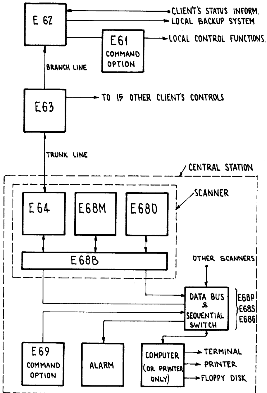
FIG. 2 . E 6800 SYSTEM
