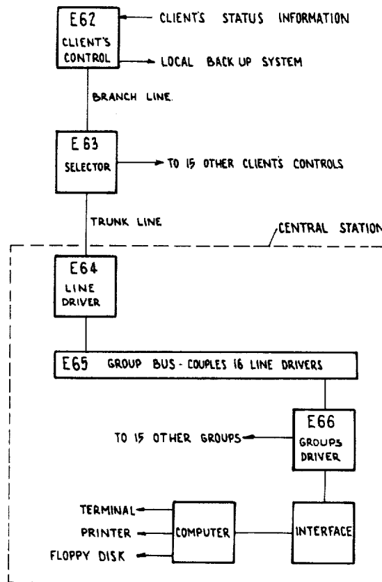
E6000 SYSTEM DIAGRAM.
