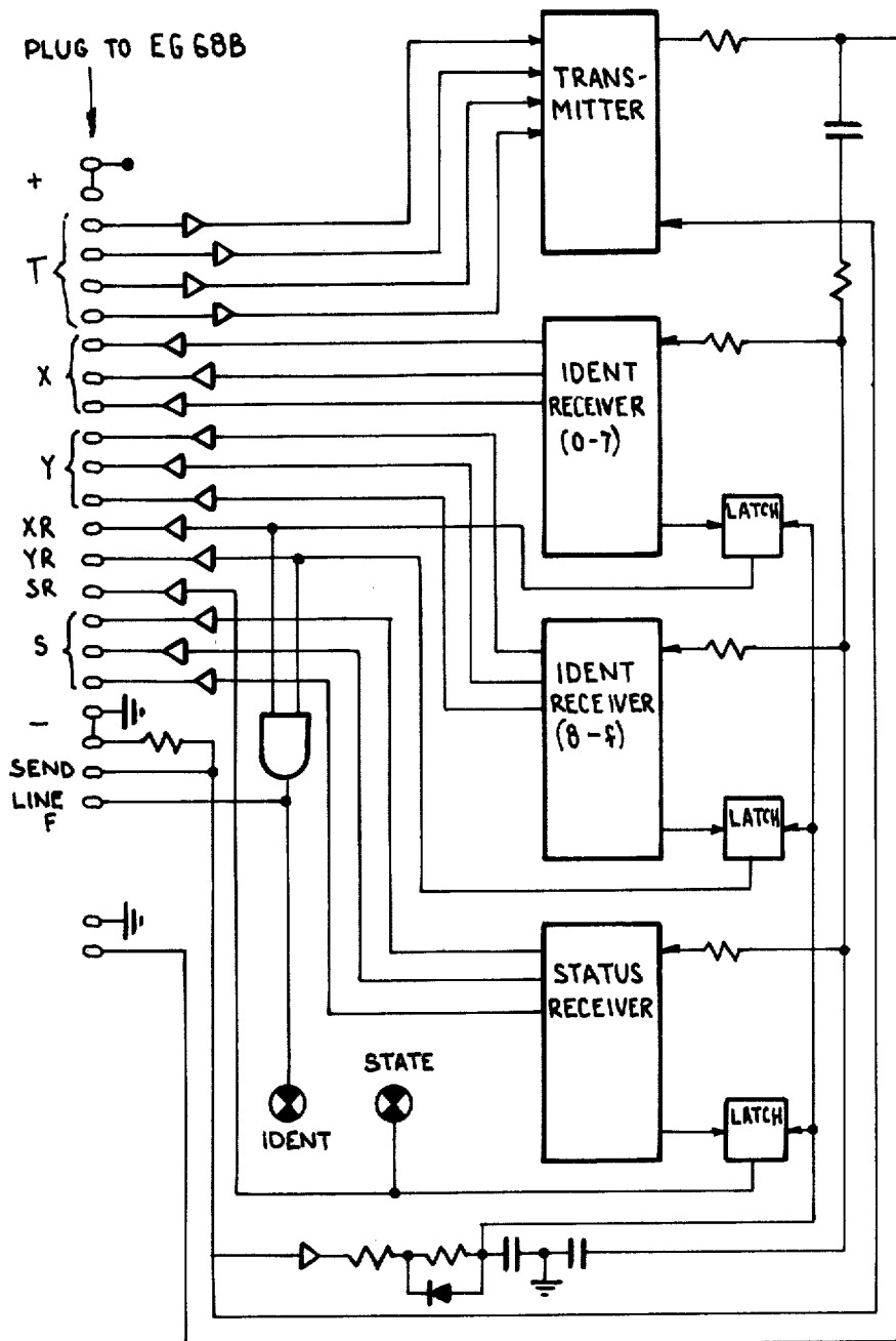
FIG. 5. E64 LINE DRIVER
