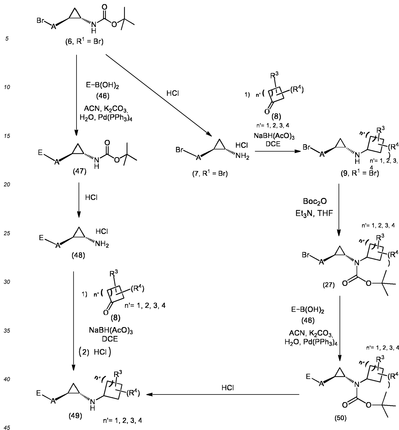
SCHEME 8: ACN (Acetonitrile), DCE (Dichloroethane), DMSO (Dimethyl sulfoxide), THF (Tetrahydrofuran)
