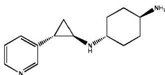
Example 83: (cis)-N1-((1R,2S)-2-(pyridin-3-yl)cyclopropyl)cyclohexane-1,4-diamine
