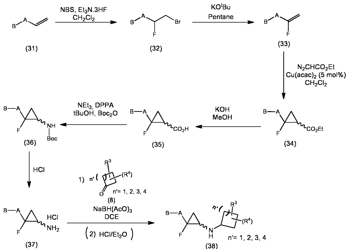
SCHEME 6: \text{Boc}_2\text{O} (Di- tert -butyl dicarbonate), DCE (Dichloroethane), DPPA (Diphenylphosphoryl azide), \text{Cu}(\text{acac})_2 (Copper(II) acetylacetonate), NBS (N-Bromosuccinimide).
