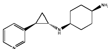
Example 82: (trans)-N1-((1R,2S)-2-(pyridin-3-yl)cyclopropyl)cyclohexane-1,4-diamine
