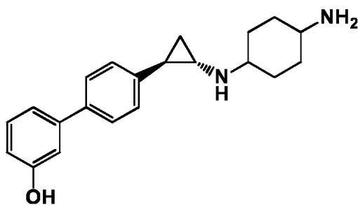
Example 63: N-(4'-((trans)-2-((4-aminocyclohexyl)amino)cyclopropyl)-[1,1'-biphenyl]-3-yl)methanesulfonamide
