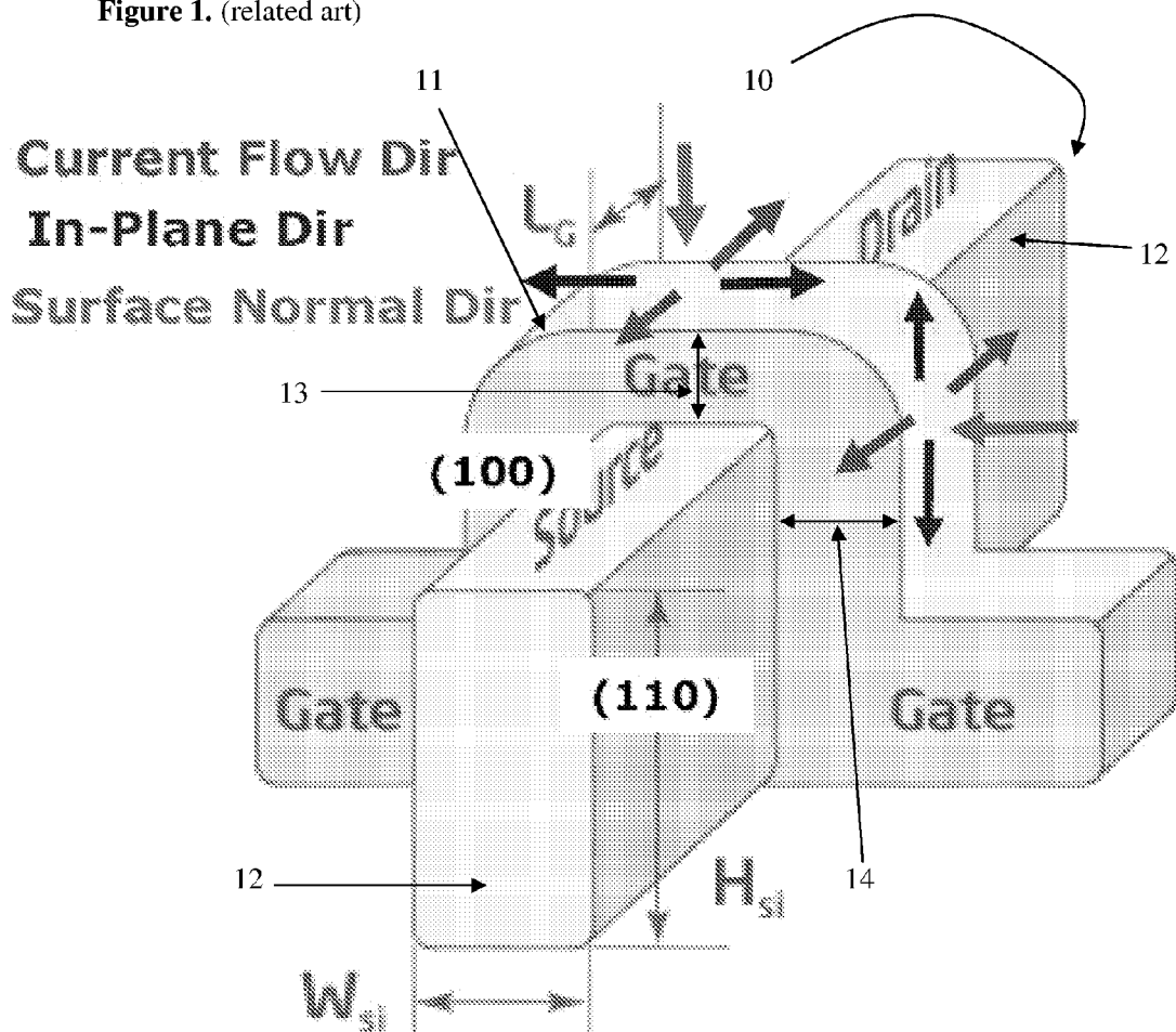
Figure 1. (related art)
