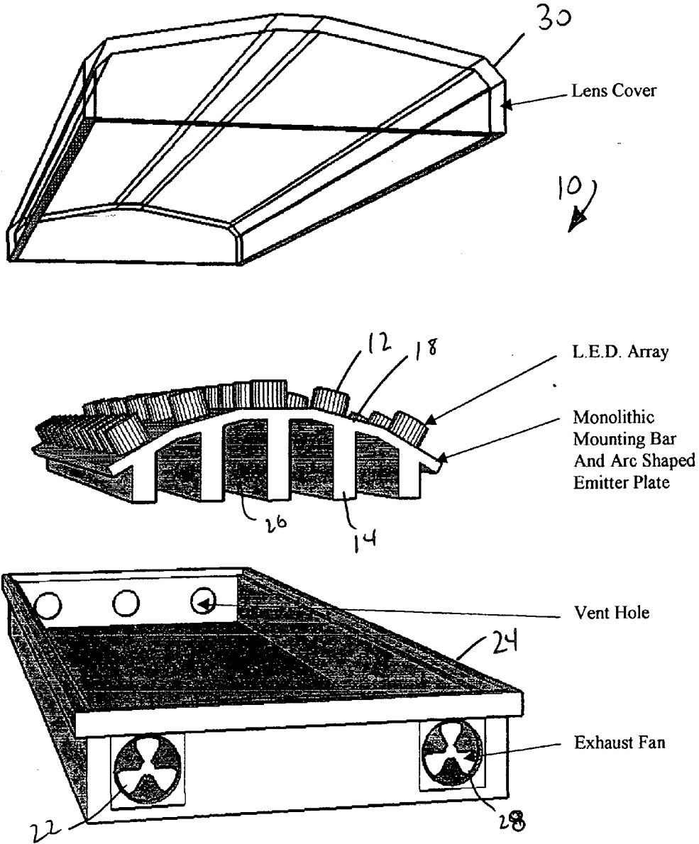
Drawing 7 - Monolithic Mounting Bar and Arc Shaped Emitter Plate
