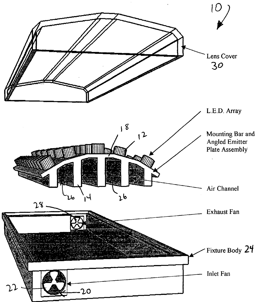
Drawing 4 – Active Cooling by Fan and Staggered Air Channels
