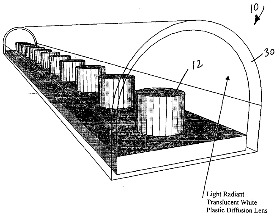
Drawing 10 - Plastic Diffusion Lens
