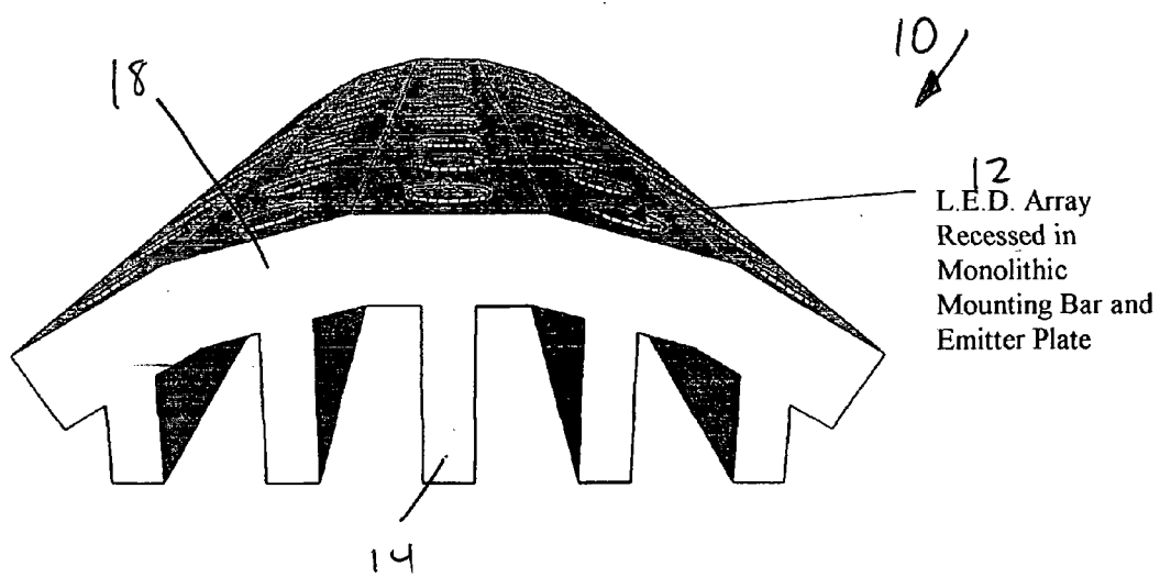
Drawing 7.1 - Recessed L.E.D. Array
