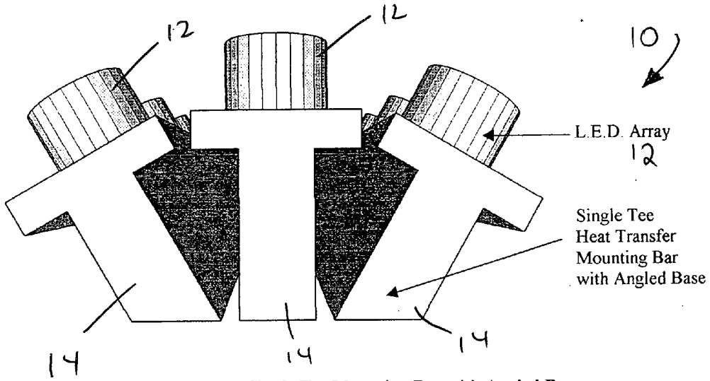
Drawing 1.1 - Single Tee Mounting Bar with Angled Base
