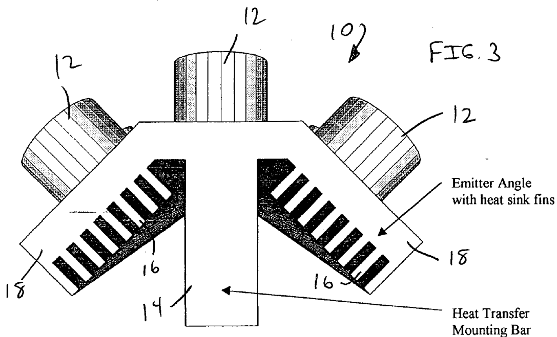
Drawing 2 - Single Tee Mounting Bar with Multiple Angled Emitter Plates
