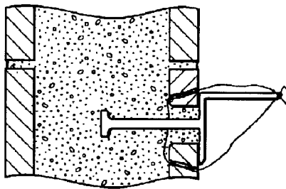
FIG. 3 PRIOR ART
