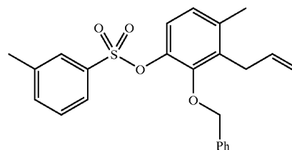
5. 4-Methyl-2-(phenylmethoxy)-3-prop-2-enylphenyl 3-methylbenzenesulfonate
