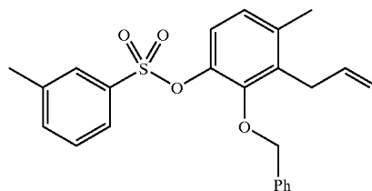
6. 4-Methyl-3-(2-oxoethyl)-2-(phenylmethoxy)phenyl 3-methylbenzenesulfonate
