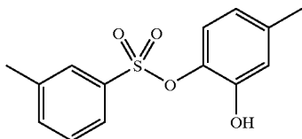
2. 2-Hydroxy-4-methylphenyl 3-methylbenzenesulfonate
