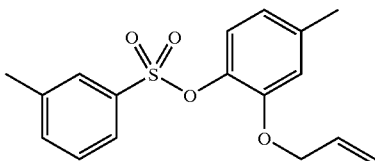
3. 4-Methyl-2-prop-2-enyloxyphenyl 3-methylbenzenesulfonate
