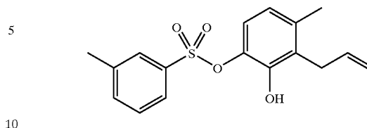
4. 2-Hydroxy-4-methyl-3-prop-2-enylphenyl 3-methylbenzenesulfonate
