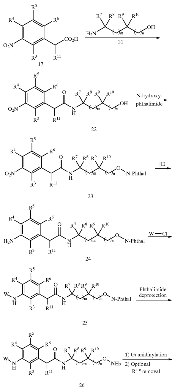
Scheme 5
