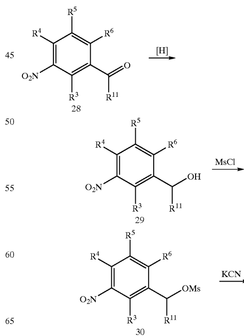
Scheme 6
