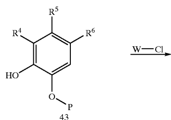
Scheme 8
