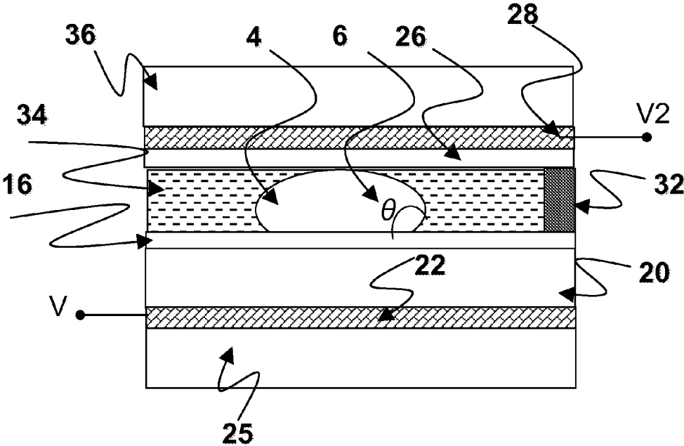
FIGURE 5: PRIOR ART
