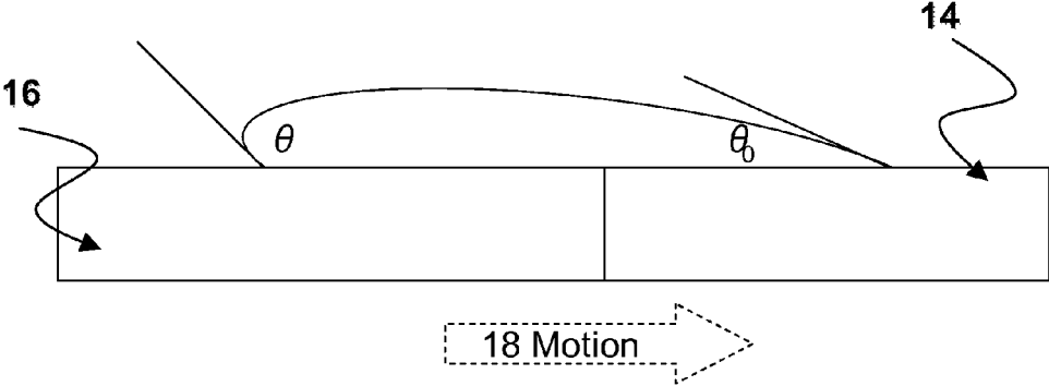
FIGURE 3: PRIOR ART
