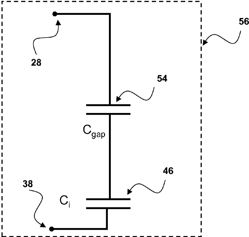
FIGURE 9: PRIOR ART
