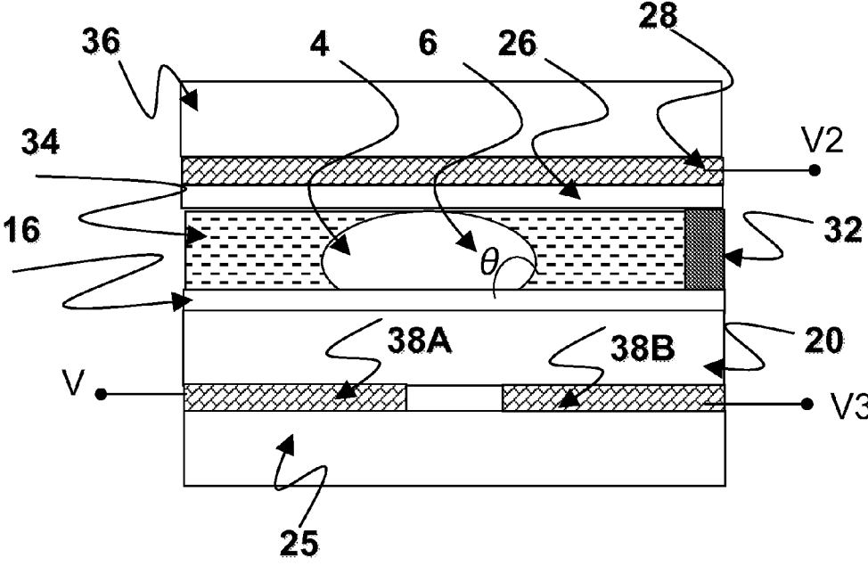
FIGURE 6: PRIOR ART
