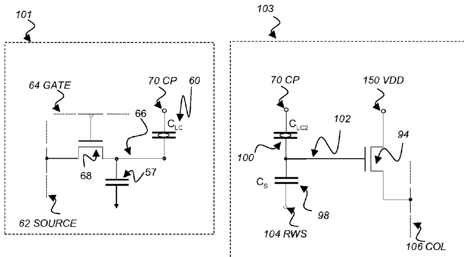
FIGURE 15: PRIOR ART
