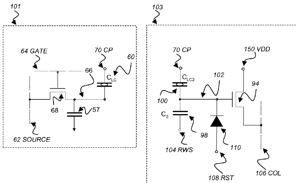
FIGURE 15: PRIOR ART
