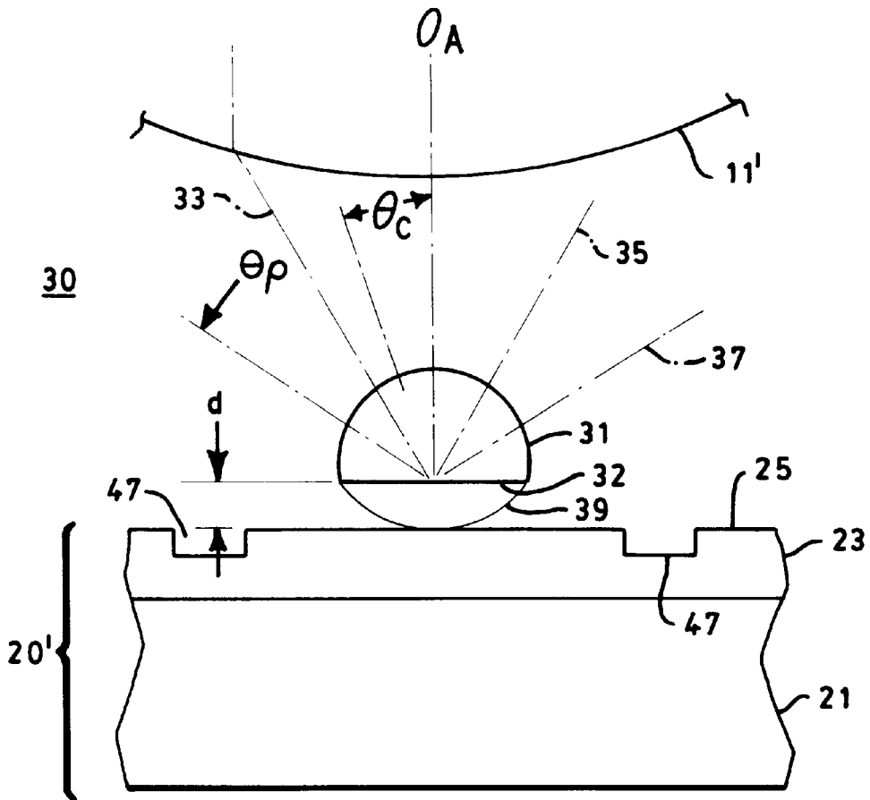
FIG. 9 (PRIOR ART)
