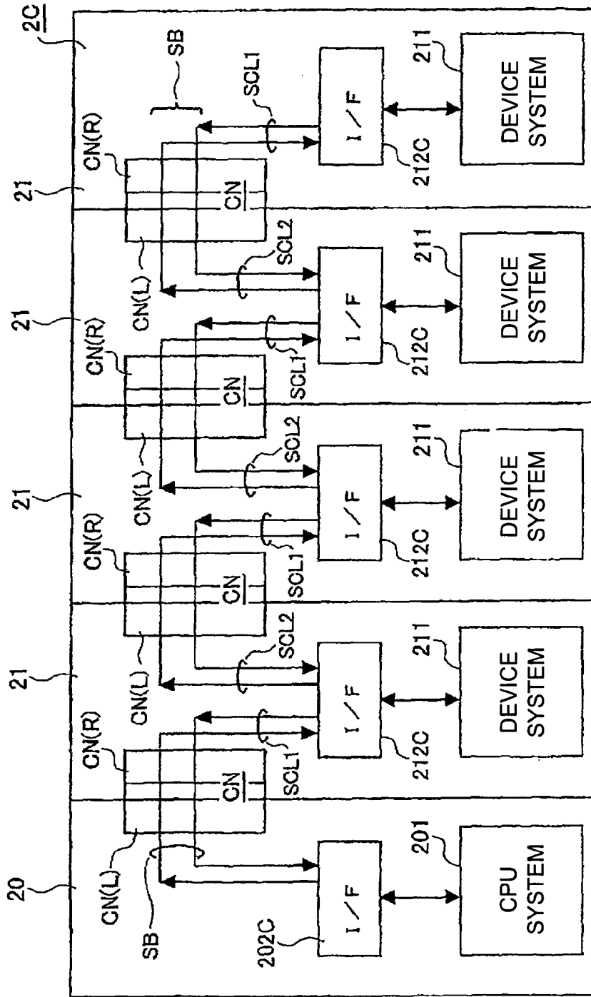
FIG. 12 (PRIOR ART)
