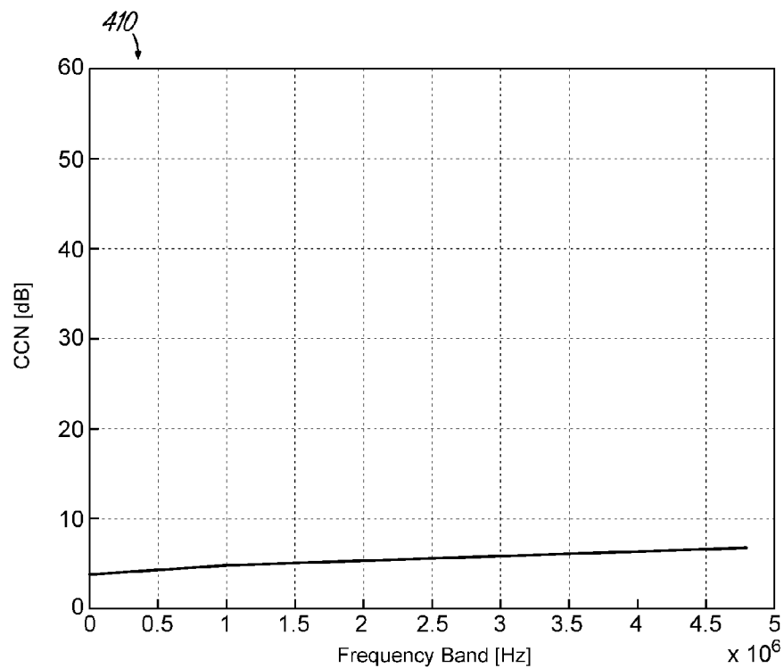
FIG.10 <5 dB Imbalance
