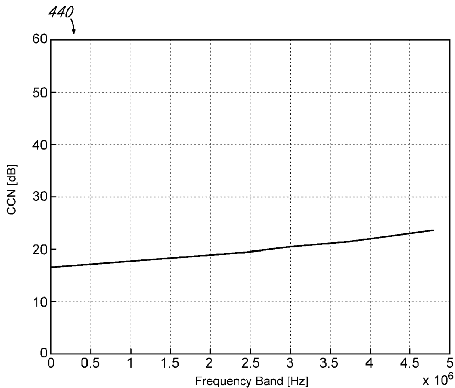
FIG.13 > 15 dB Imbalance
