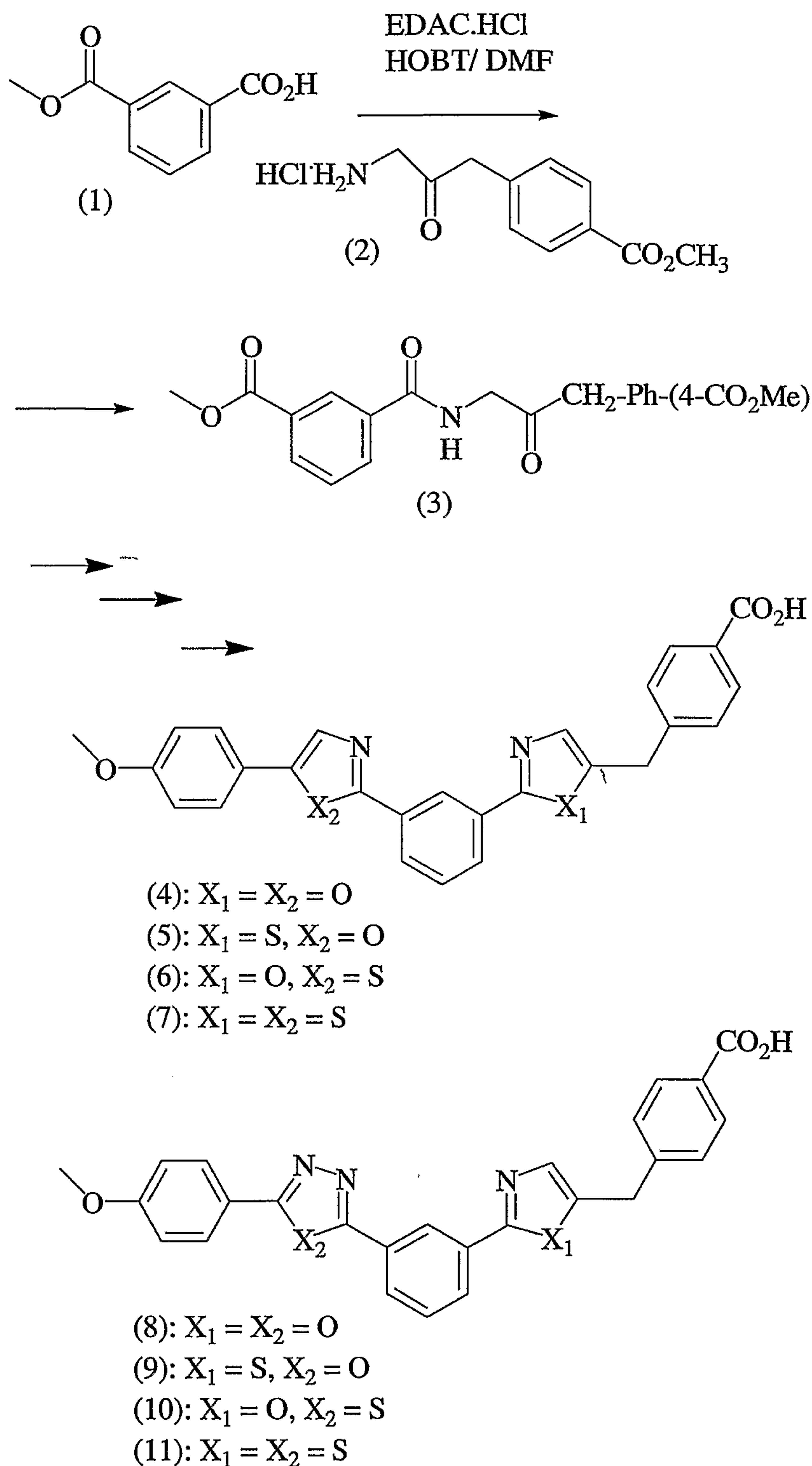
Scheme 10.
