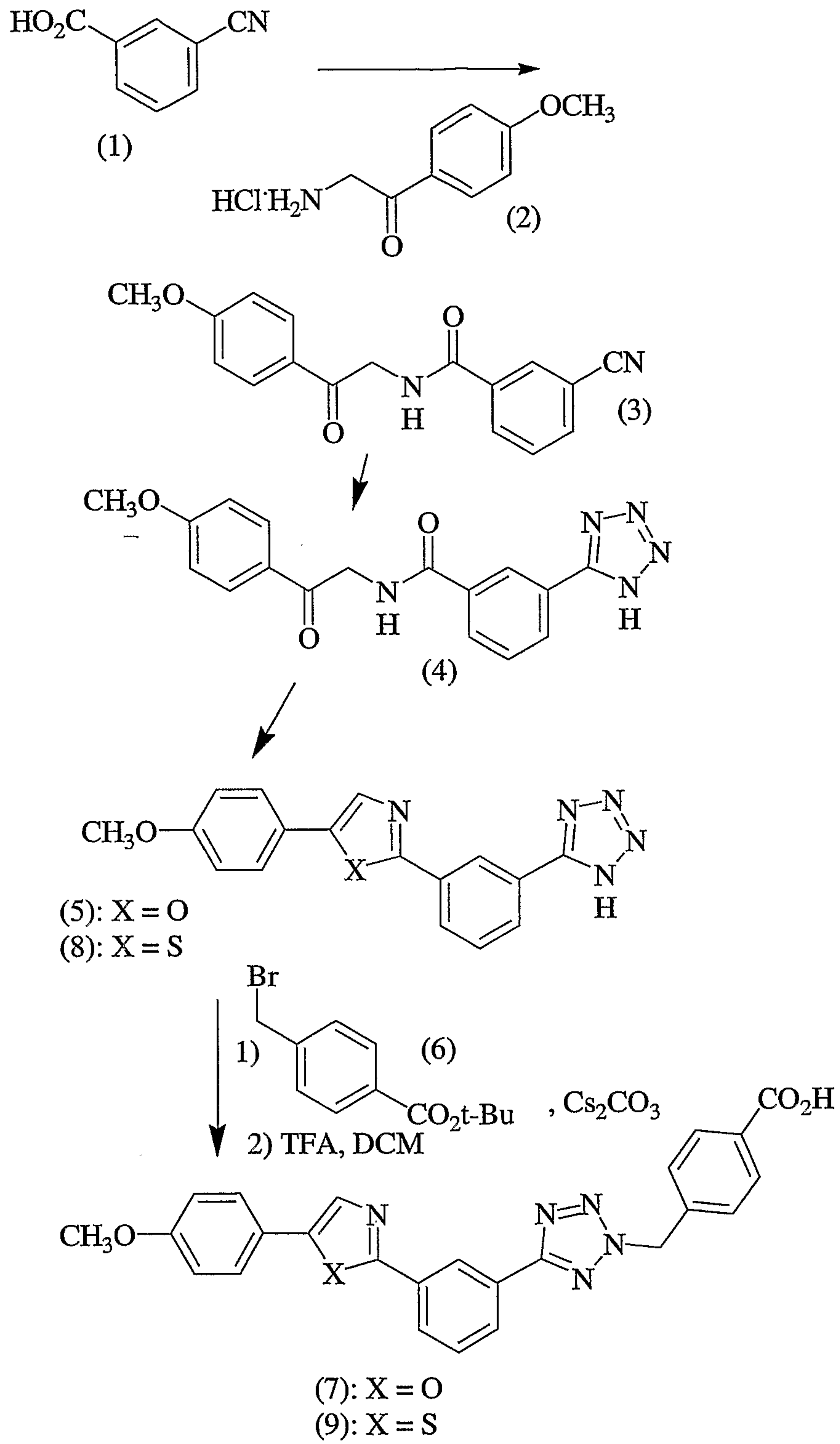
Scheme 8.
