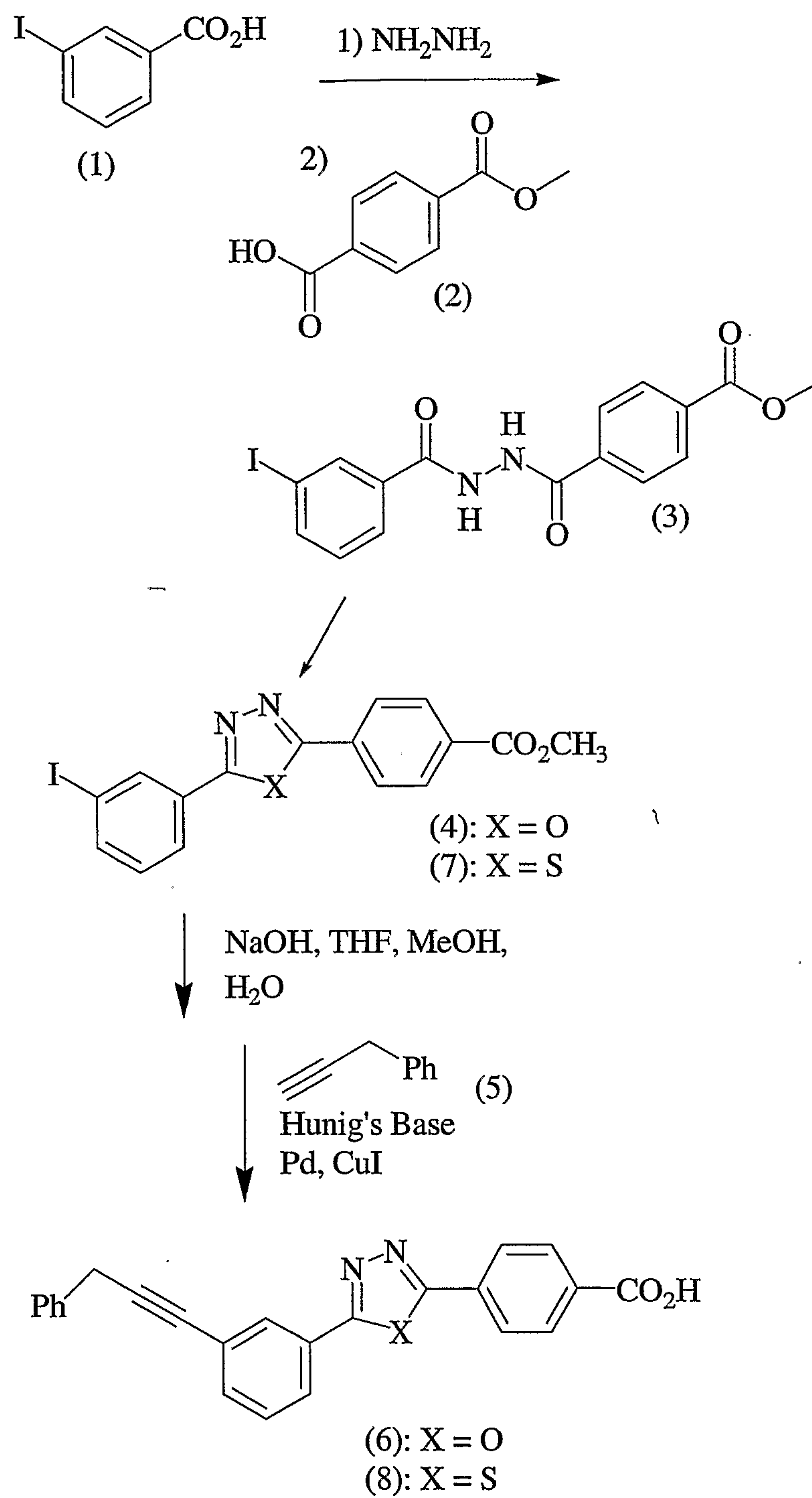
Scheme 7.
