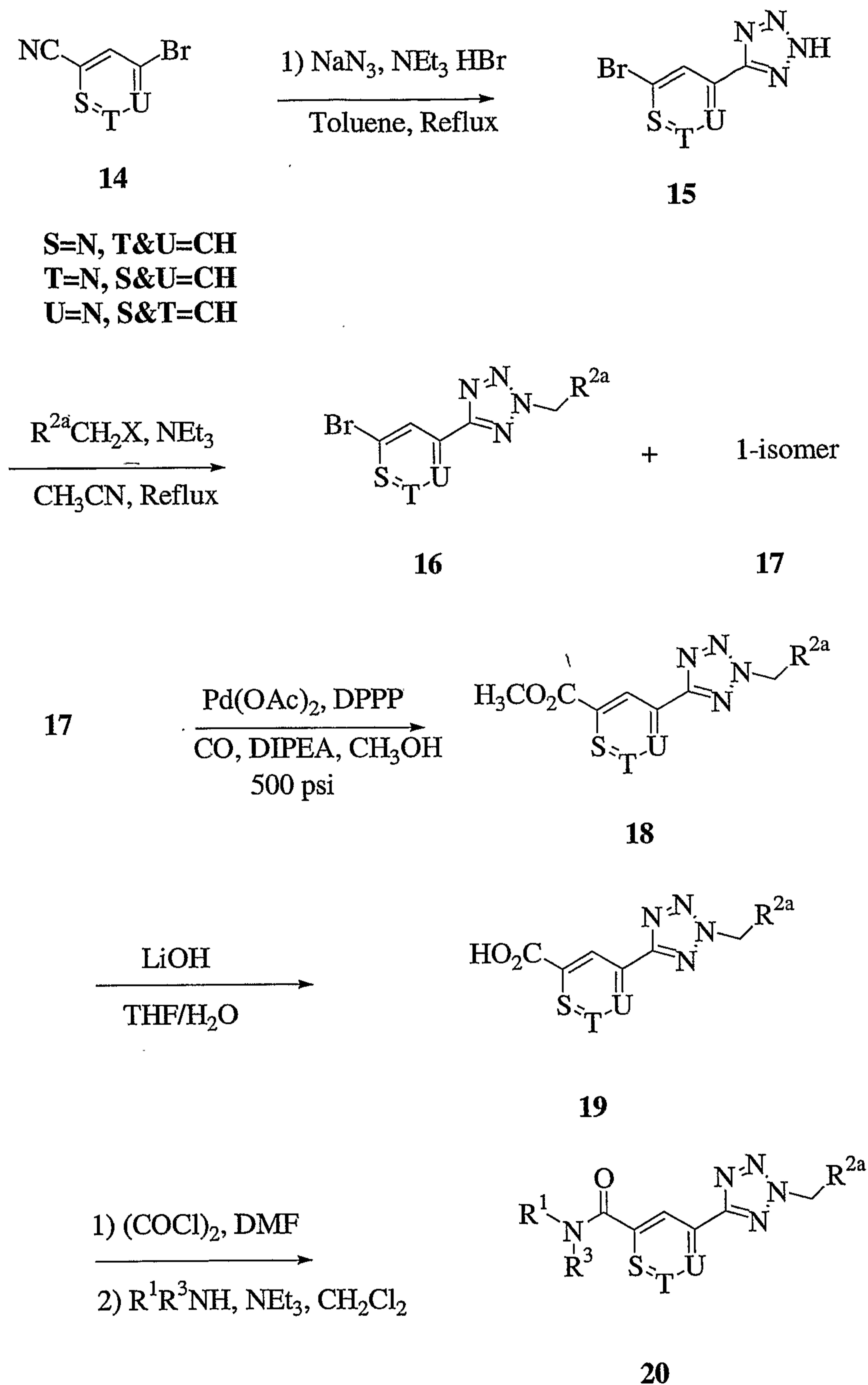
Scheme 3.
