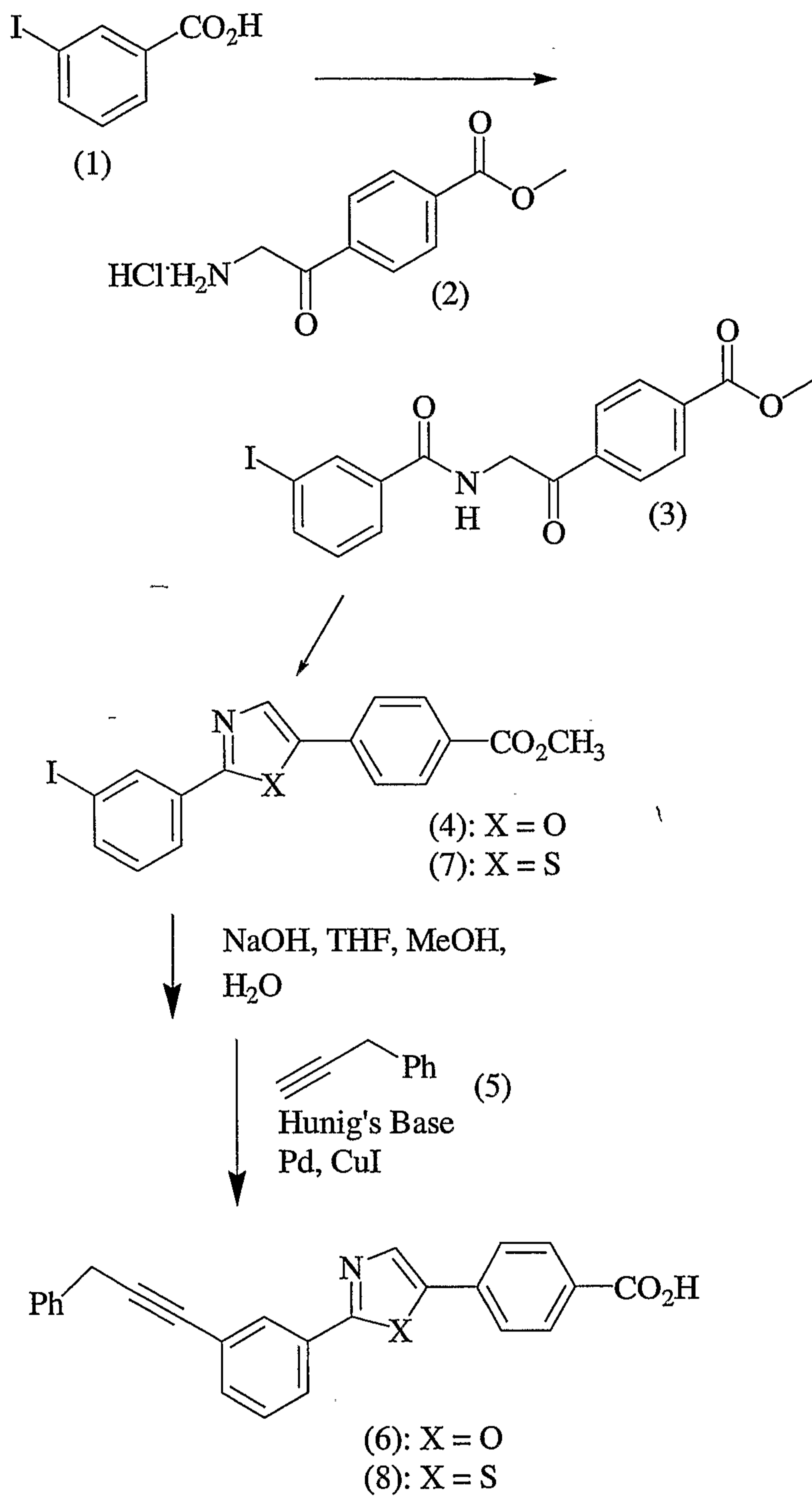
Scheme 6.
