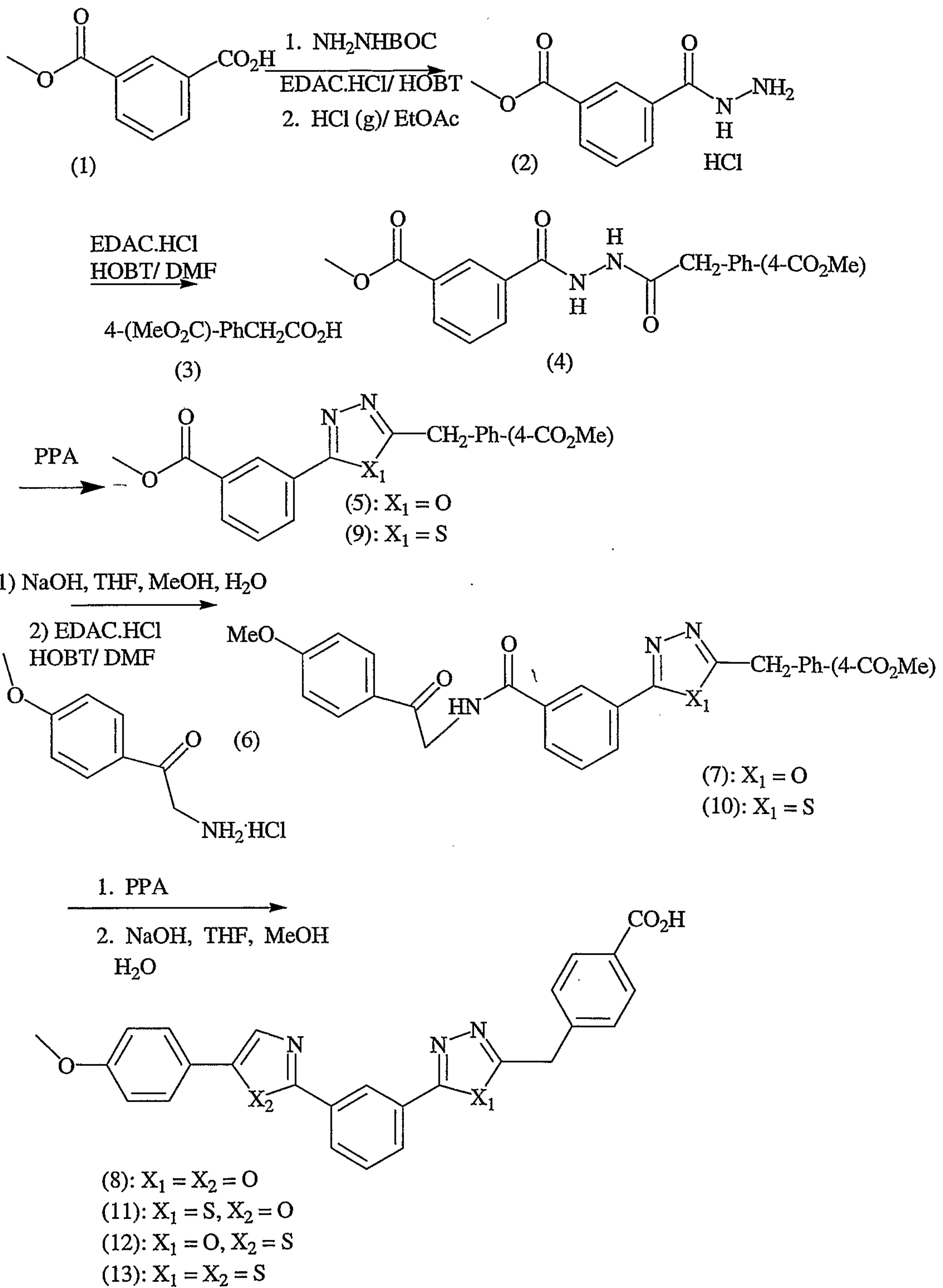
Scheme 9.
