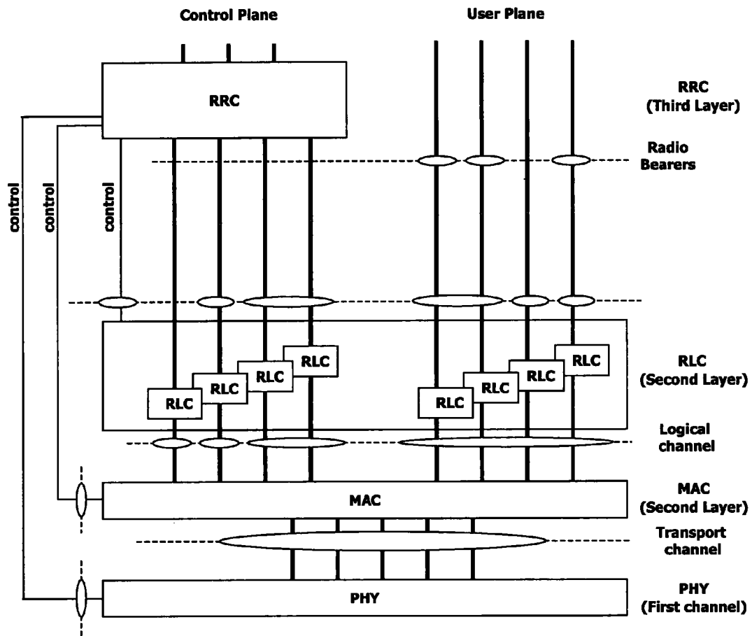
FIG. 2 RELATED ART
