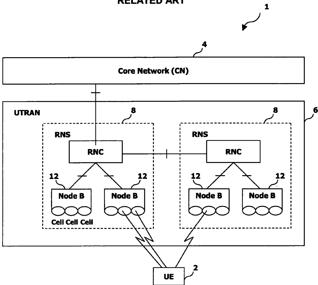
FIG. 1 RELATED ART
