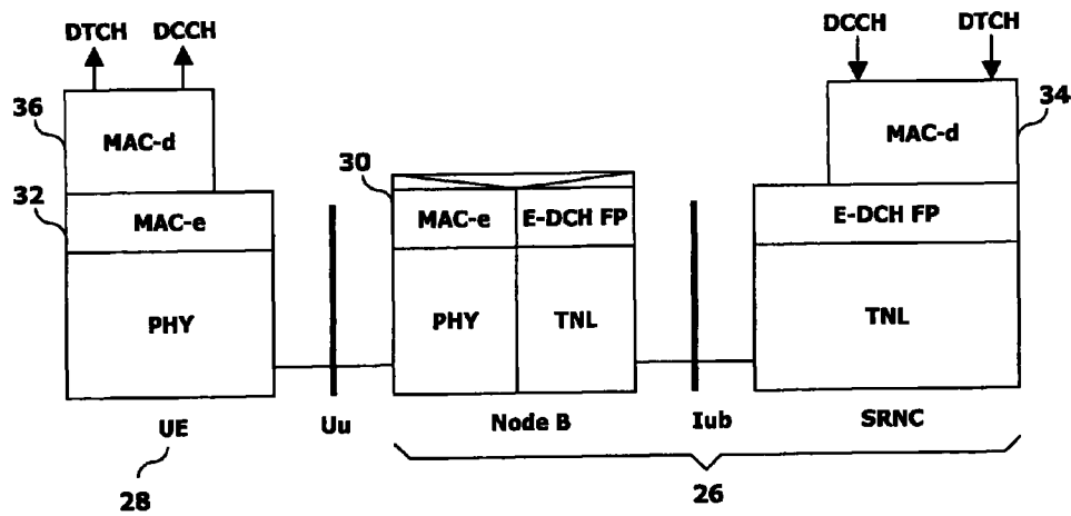
FIG. 4 RELATED ART
