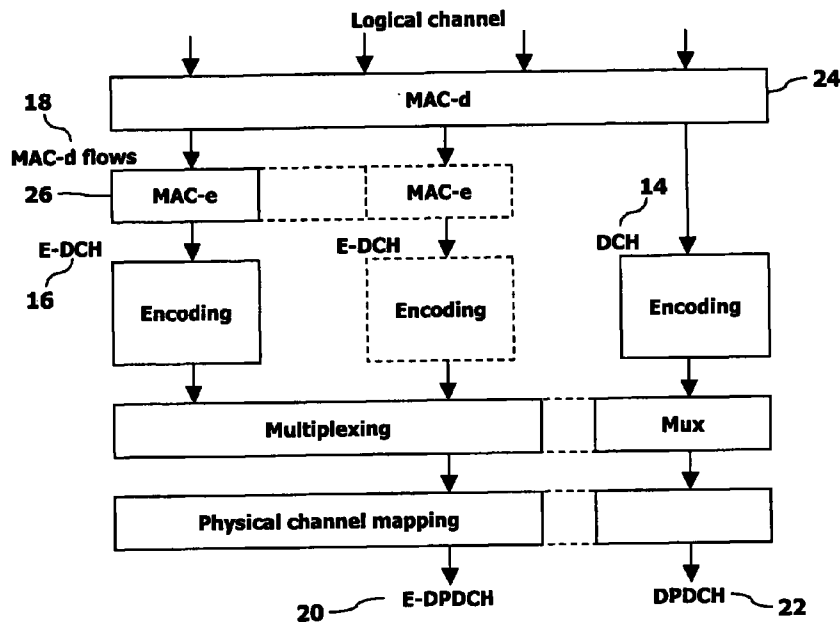
FIG. 4 RELATED ART
