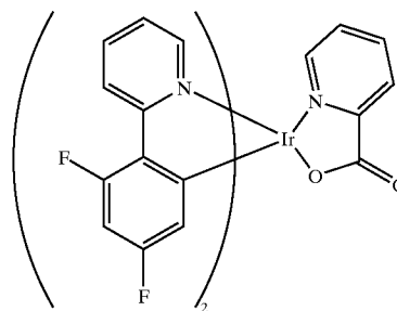
bis(2-(4,6-difluorophenyl)pyridyl-N, C2')iridium(III) picolinate (FIrpic)
