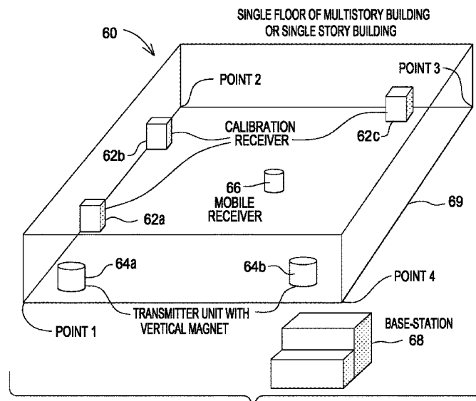
PERSONNEL TRACKING SYSTEM
