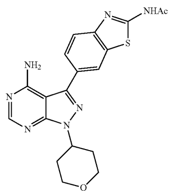
Compound 19
