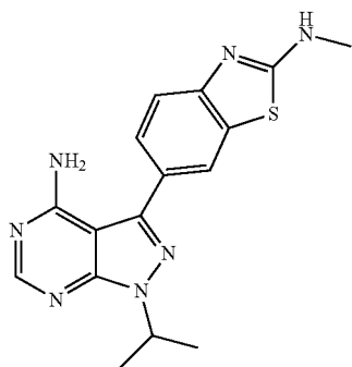
Compound 11
