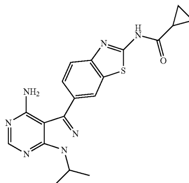
Compound 8
