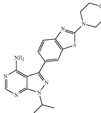
Compound 14
