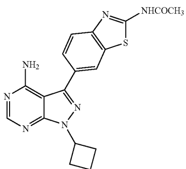
Compound 10
