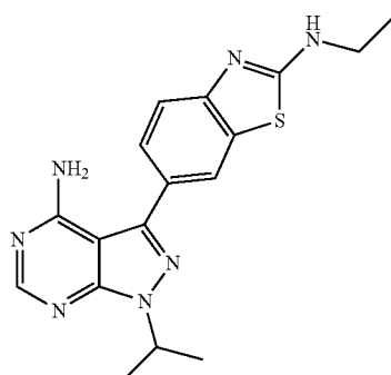
Compound 12
