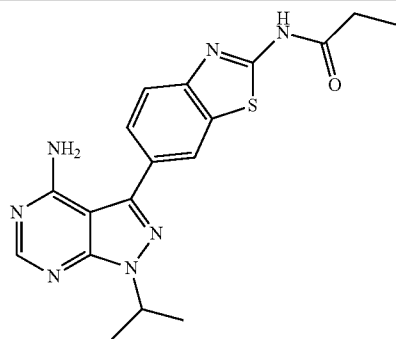
Compound 9
