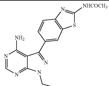
Compound 5
