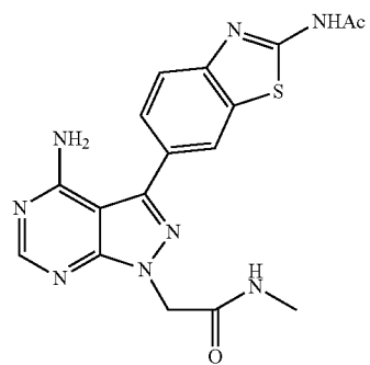
Compound 18
