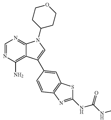
Compound 21
