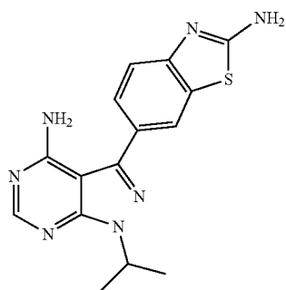
Compound 3
