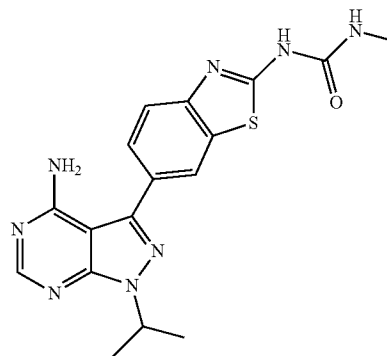
Compound 20
