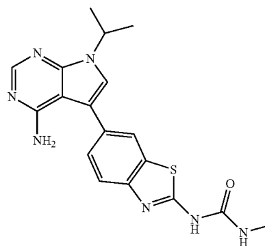
Compound 22
