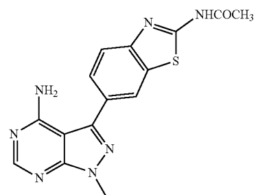
Compound 6
