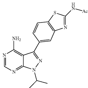
Compound 17
