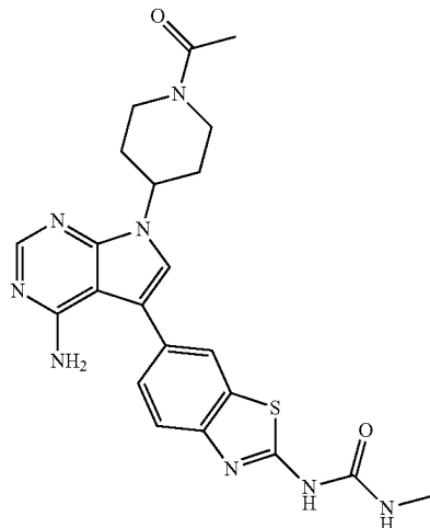
Compound 23
