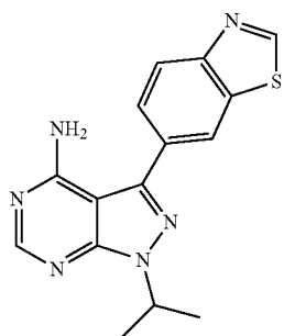
Compound 2
