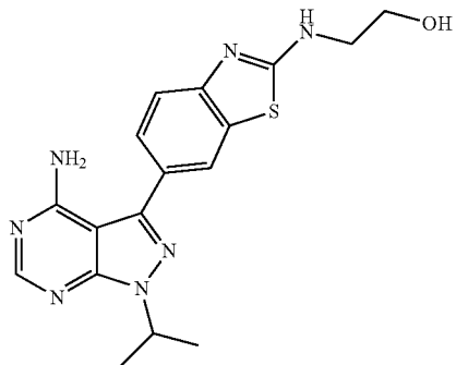
Compound 16
