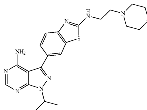
Compound 13
