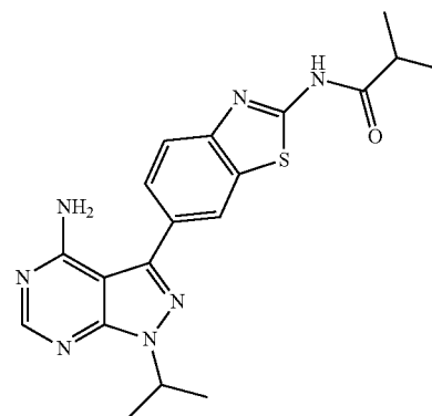
Compound 7
