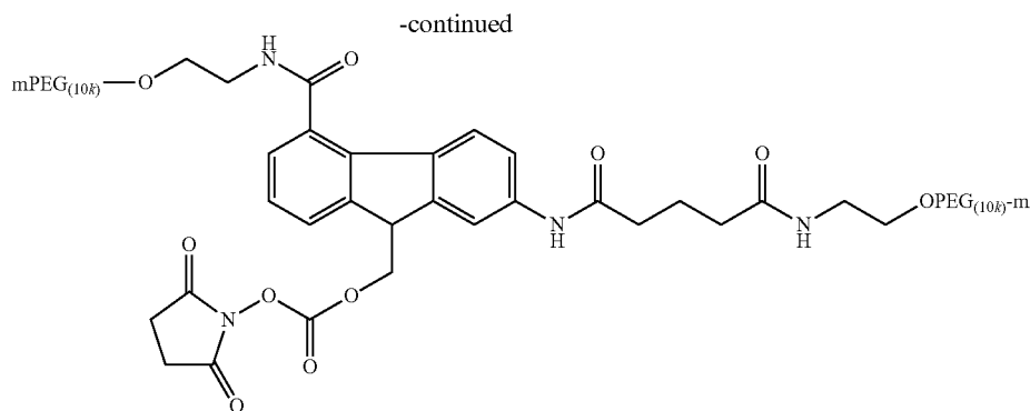
9-hydroxymethyl-4-(mPEG(10,000)-carboxamide)-7-(mPEG(10,000)-amidoglutaric acid)fluorene-N-hydroxysuccinimide
