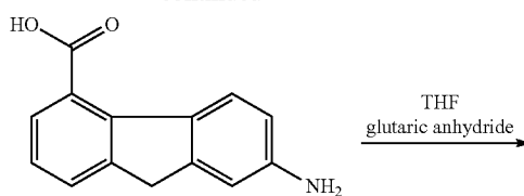
4-carboxylic acid-7-aminofluorene
