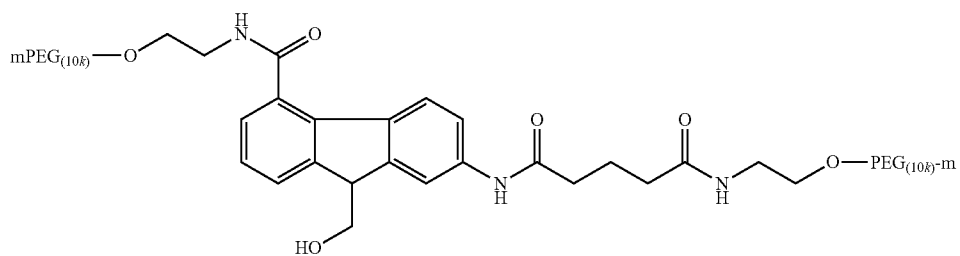
9-hydroxymethyl-4-(mPEG(10,000)-carboxyamide)-7-(mPEG(10,000)-amidoglutamic acid)fluorene
