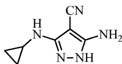
5-amino-3-(cyclopropylamino)-1H-pyrazole-4-carbonitrile
