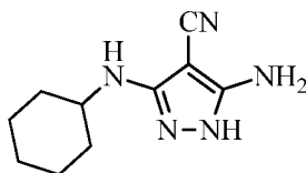
5-amino-3-(cyclohexylamino)-1H-pyrazole-4-carbonitrile
