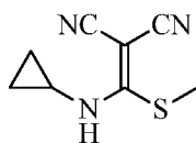
2-((cyclopropylamino)(methylthio)methylene)malononitrile
