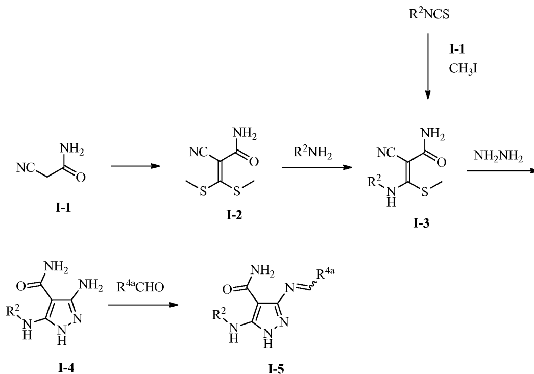
Scheme I
