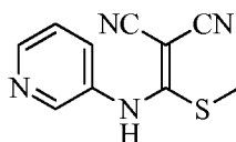
2-((methylthio)(pyridin-3-ylamino)methylene)malononitrile
