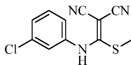
2-(((3-chlorophenyl)amino)(methylthio)methylene)malononitrile
