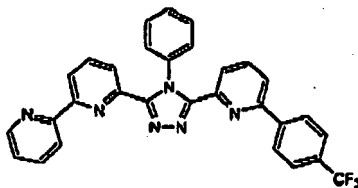
(Compound 5)
