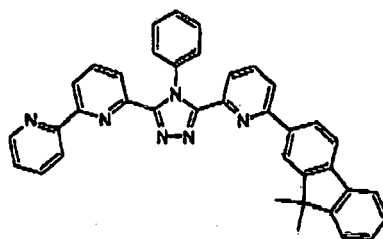
(Compound 16)
