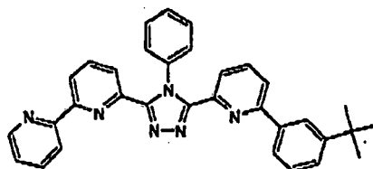
(Compound 3)
