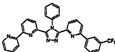
(Compound 6)
