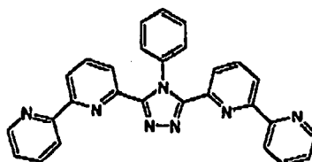
(Compound 17)
