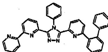
(Compound 15)
