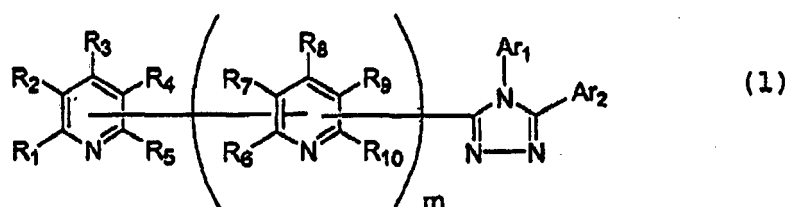
[Chem. 2]
