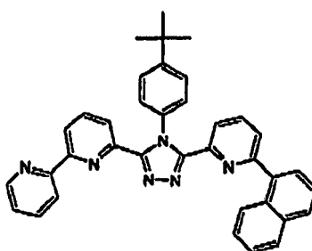
(Compound 24)
