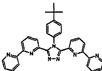
(Compound 26)
