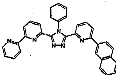
(Compound 10)
