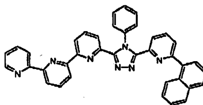
(Compound 31)
