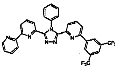
(Compound 7)
