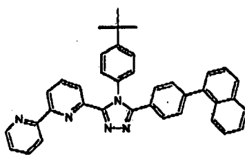
(Compound 27)
