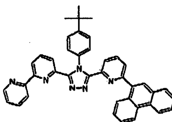
(Compound 25)
