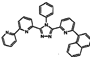
(Compound 9)
