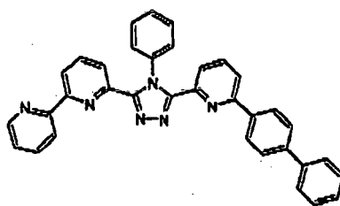
(Compound 13)
