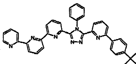
(Compound 29)
