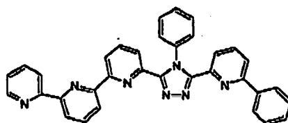
(Compound 30)
