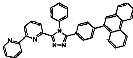
(Compound 22)
