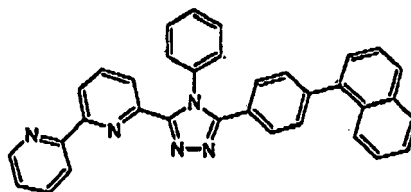
(Compound 21)
