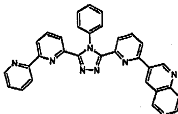
(Compound 19)
