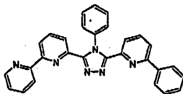
(Compound 4)
