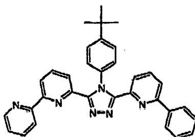
(Compound 23)
