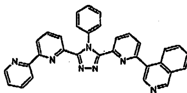
(Compound 18)
