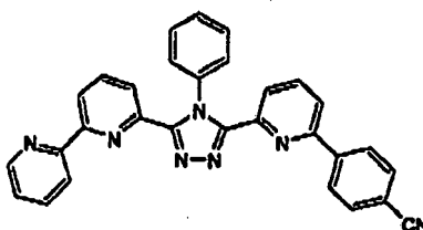
(Compound 8)
