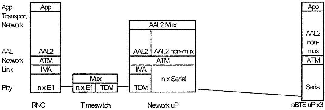
UMTS '99 (ATM backhaul) User Flow
