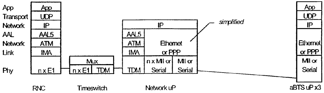
UMTS '00 (IPoA backhaul) User Flow / CDMA A.bis User Traffic
