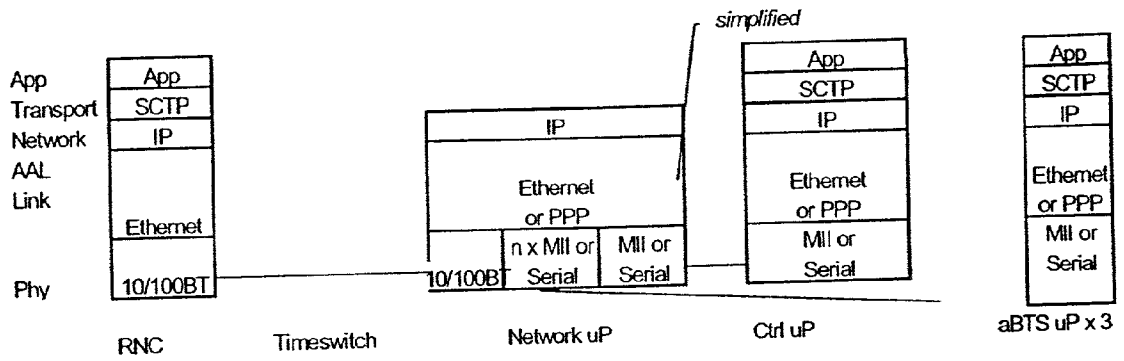
UMTS '00 (IP/Ethernet backhaul) NBAP Flow / CDMA A.bis
