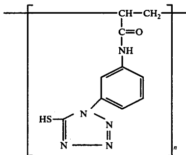
poly[1-(m-(2-acrylamido-2-methyl)-propionamido-phenyl)-1,2,3,4-tetrazole-5-thiol],
