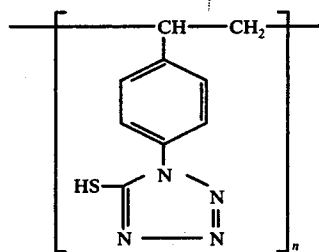
poly[1-(p-vinylbenzyl)-1,2,3,4-tetrazole-5-thiol],
