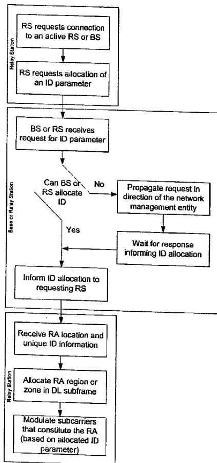
Interaction between a network associating RS and the already operational network.
