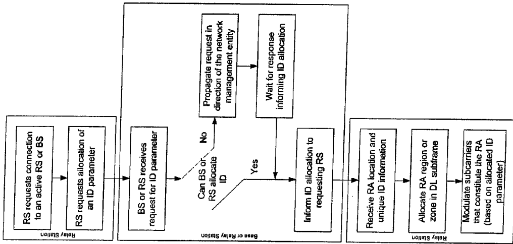
Figure 4: Interaction between a network associating RS and the already operational network.
