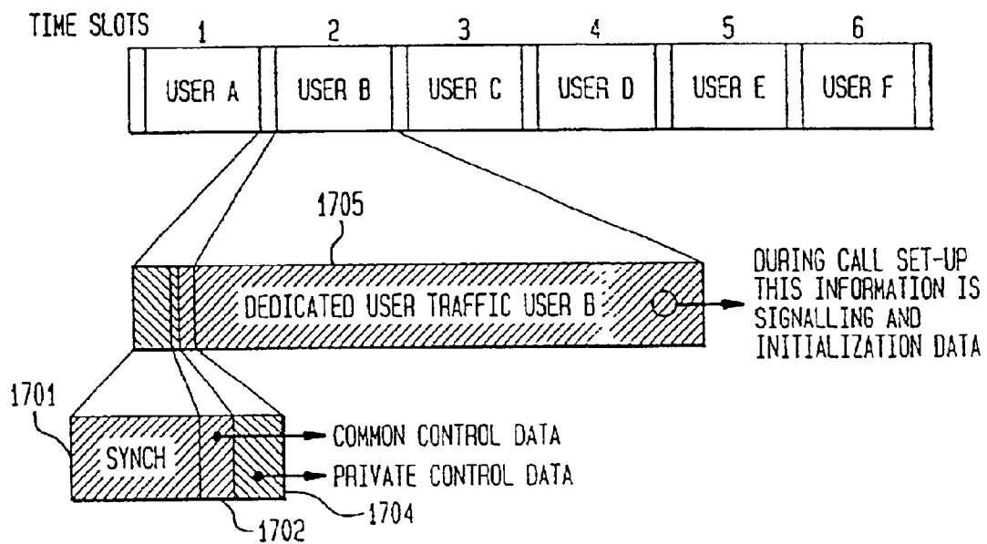
SYNCH AND CONTROL CHANNEL STRUCTURE
