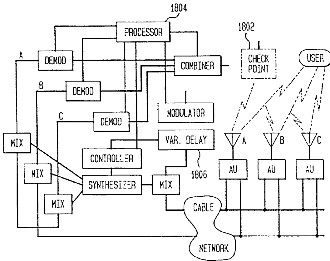
TIME CALIBRATION FOR DISTRIBUTED ANTENNA IMPLEMENTATION
