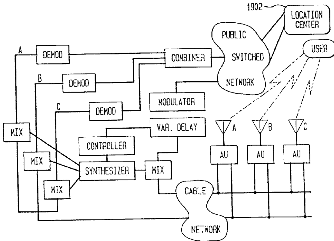
FIG. 19 LOCATION CENTER EXTERNAL TO COMMUNICATION SYSTEM
