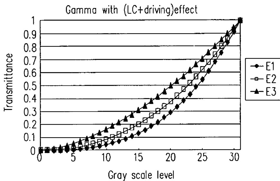
FIG. 5 (PRIOR ART)
