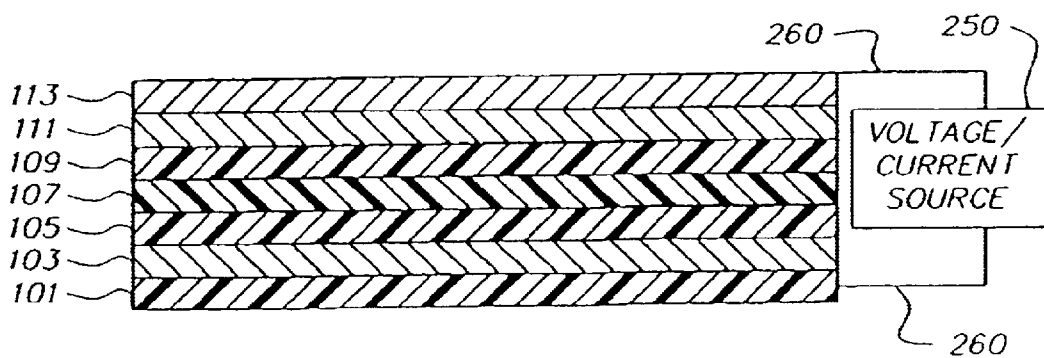
FIG. 3 (PRIOR ART)
