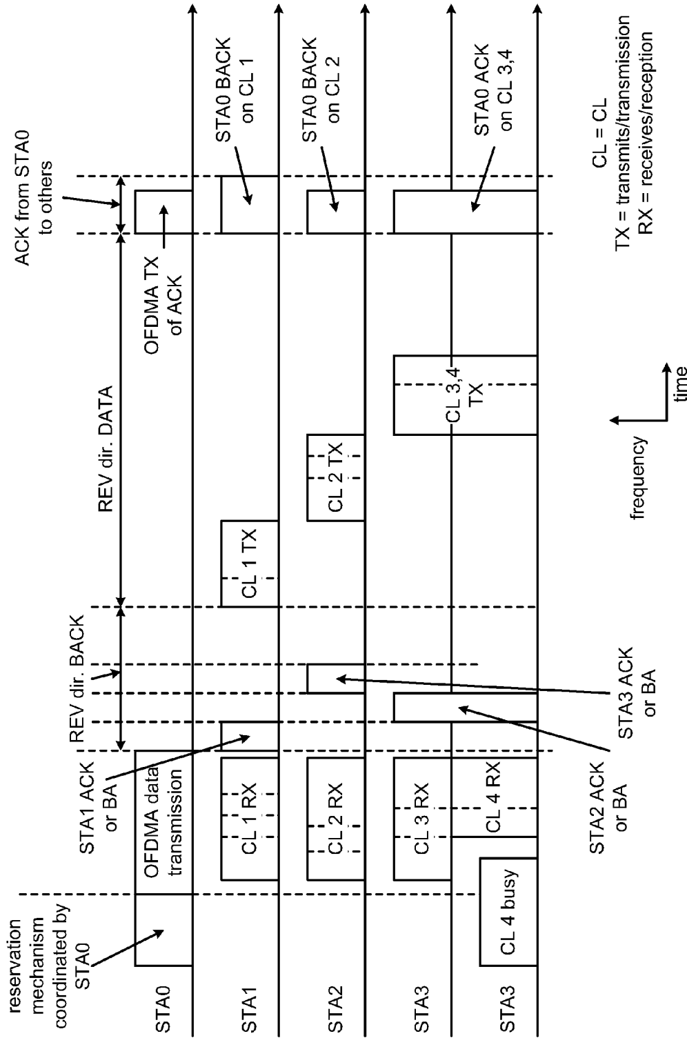
MU-SF timing - using newly available cluster (21)
