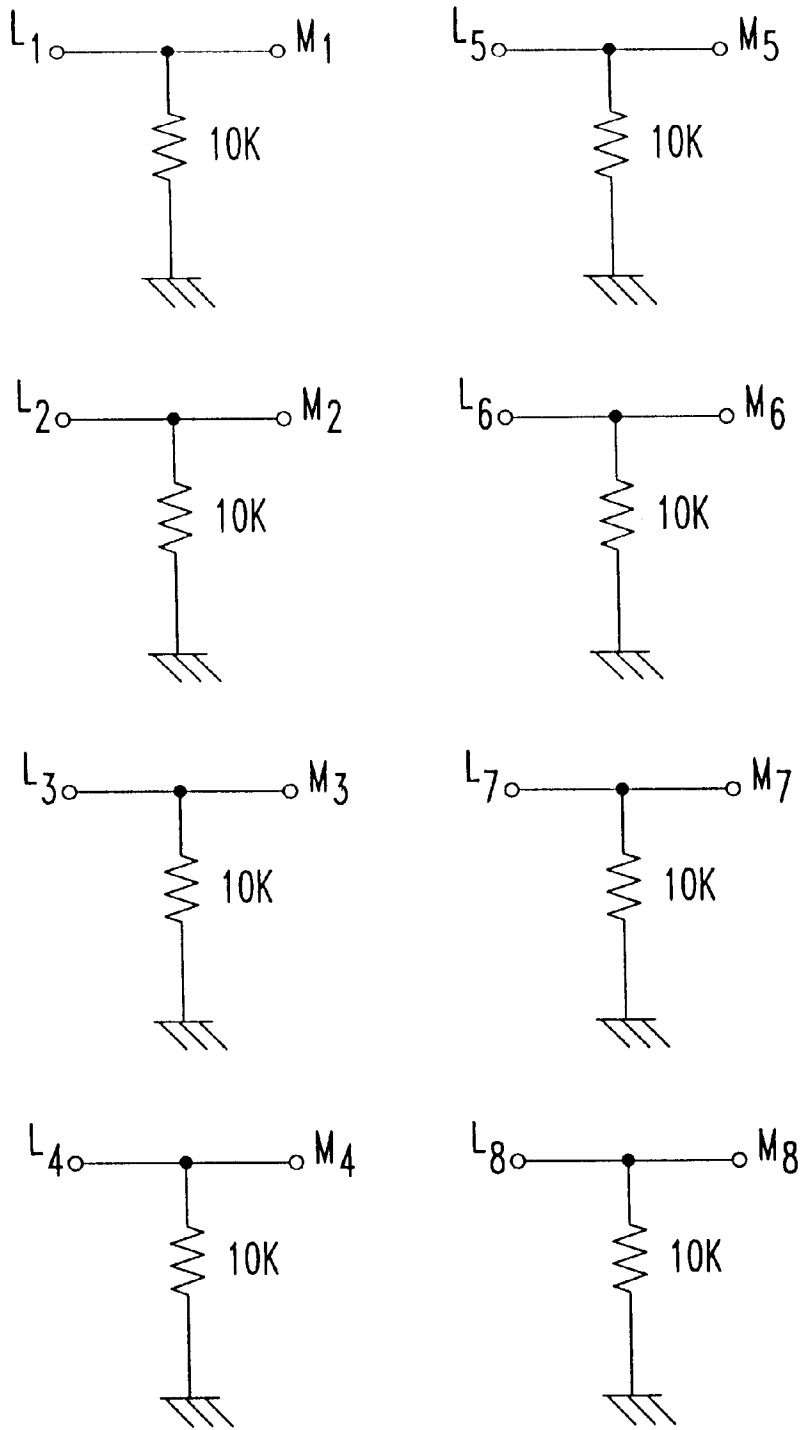
OUTPUT MUX LOAD RESISTORS
