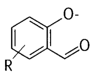
salicylaldehydes
