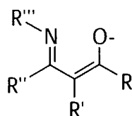
iminoacetates
