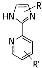
pyridylimidazoles
