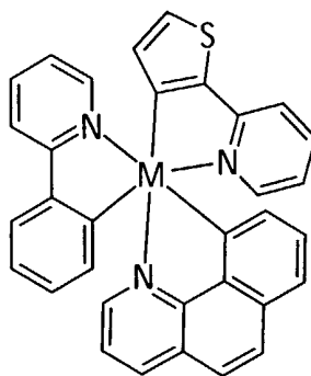
M(ppy)(bq)(thpy)
