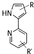
pyridylpyroles
