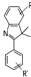
phenylindoles
