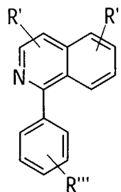
arylquinolines
