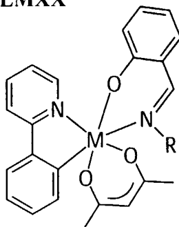
M(ppy)(sd)(acac)
