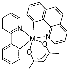
M(ppy)(bq)(acac)
