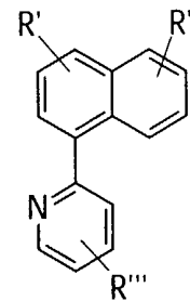
pyridynaphthalenes
