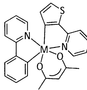
M(ppy)(thpy)(acac)
