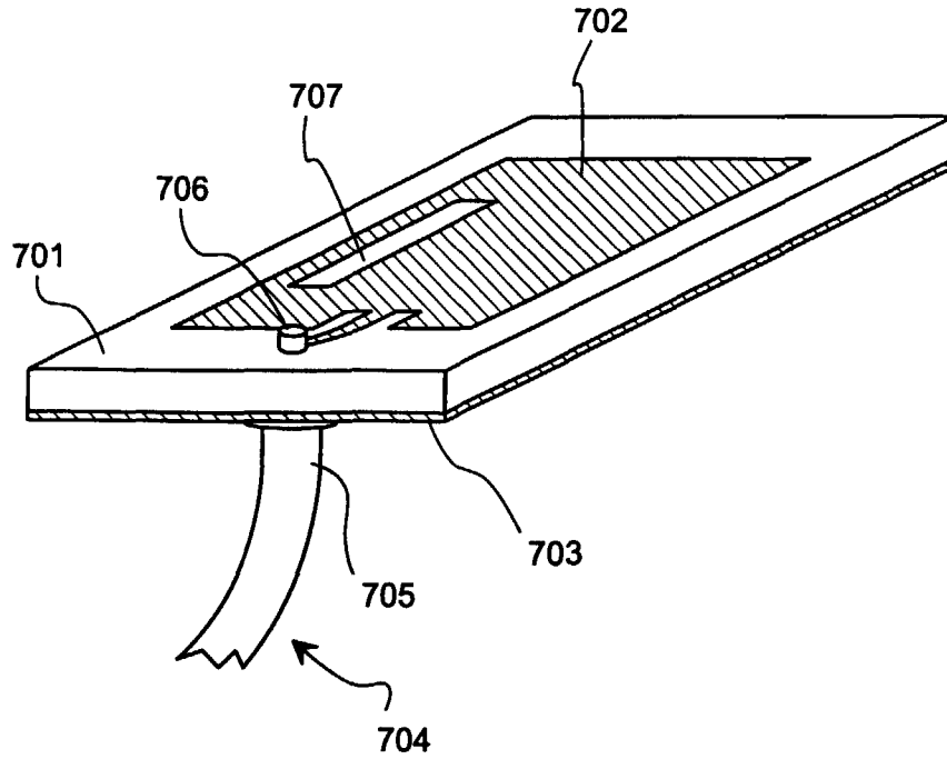
Fig. 7 PRIOR ART
