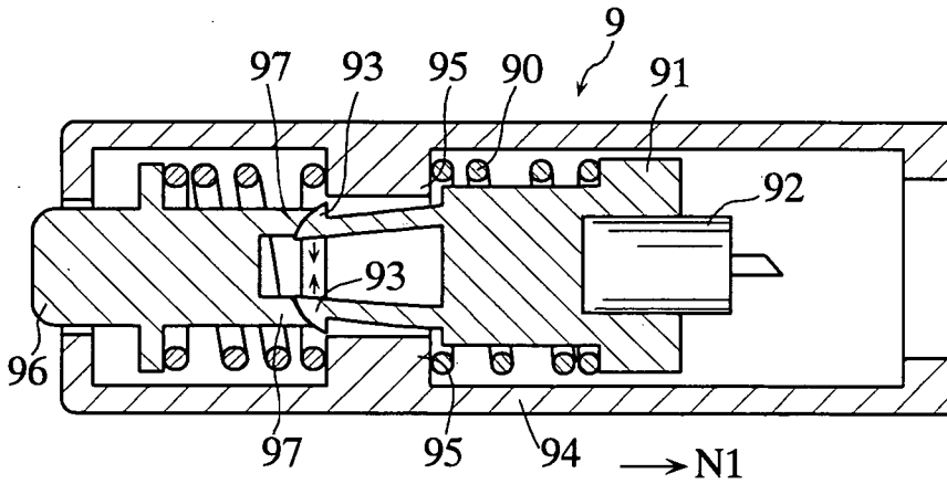
FIG.32C PRIOR ART
