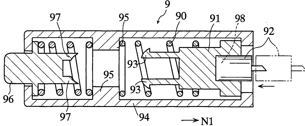
FIG.32C PRIOR ART
