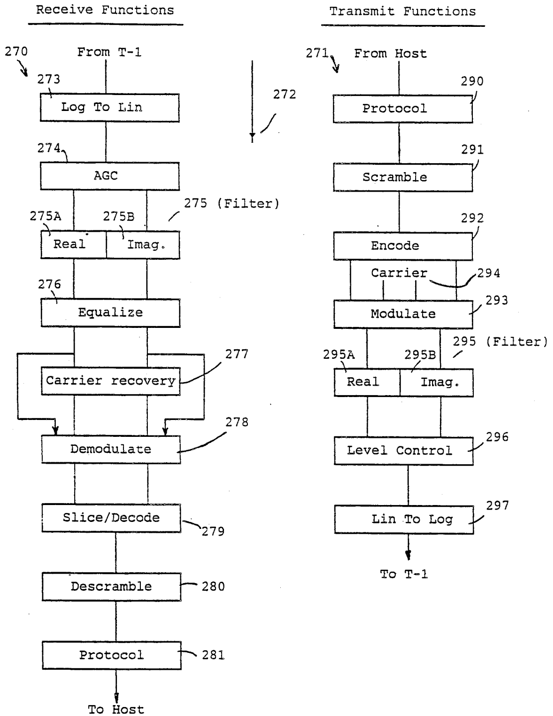
Fig. 15 (Example of Coherent Phase Shift Keyed Modem)
