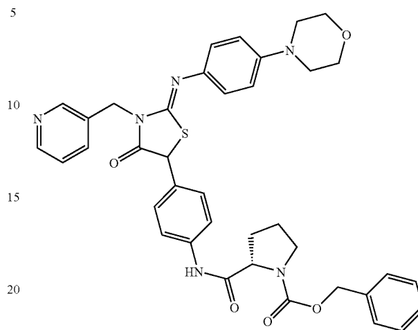
Compound 81 NS5A Inhibitor
