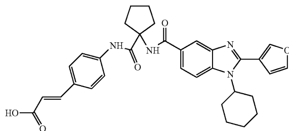
Replicase Inhibitor cmpd 2006 of WO 03/010141
