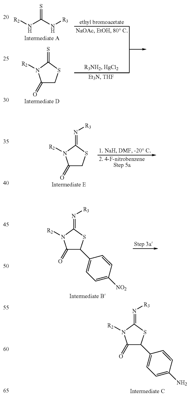
General Synthetic Scheme 2
