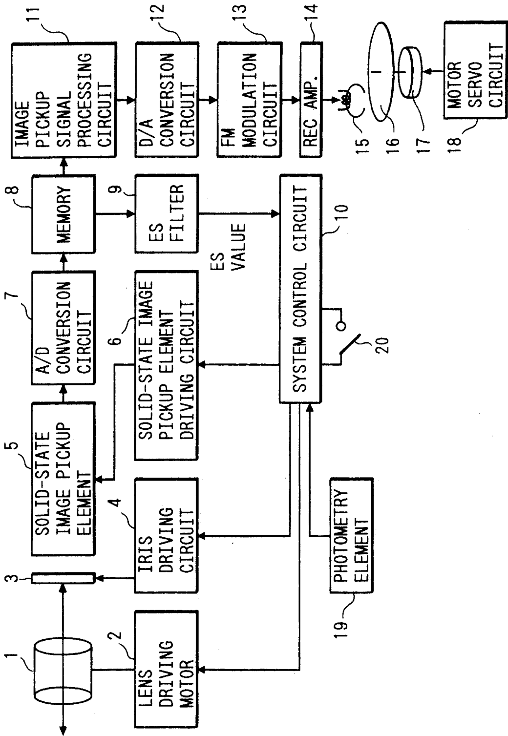
FIG. 1 (PRIOR ART)
