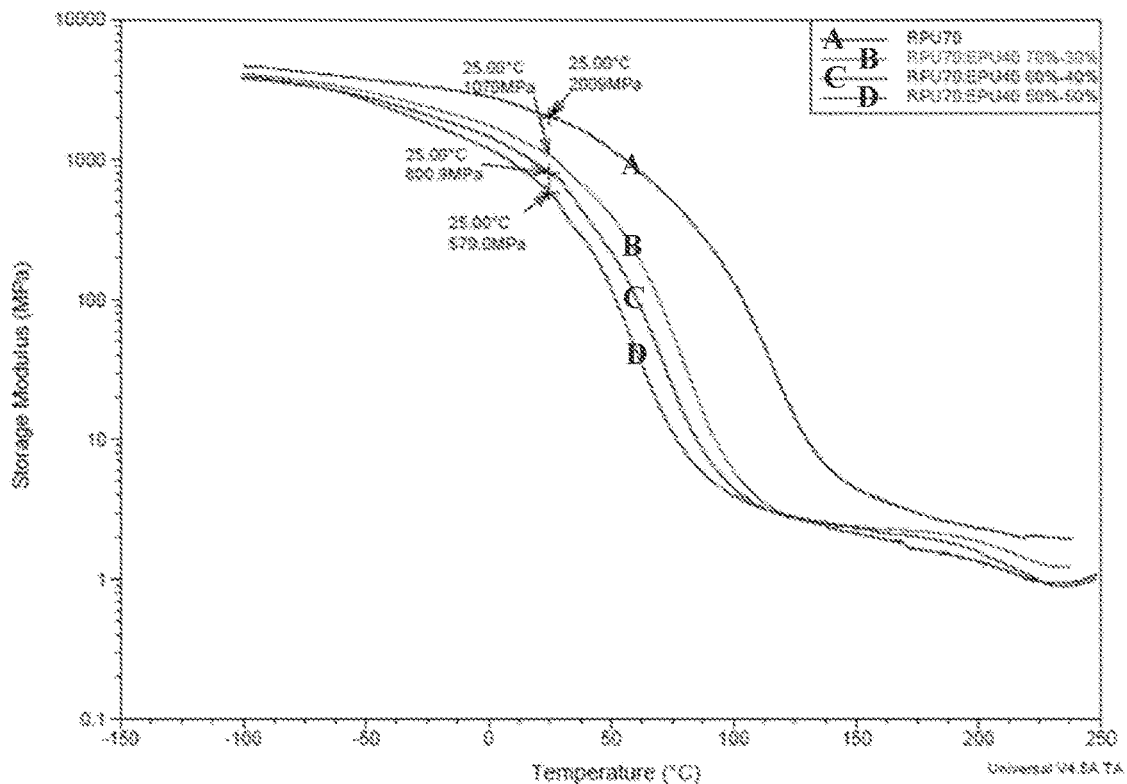
Figure 7: RPU70 + EPU40 Room Temperature Storage Modulus
