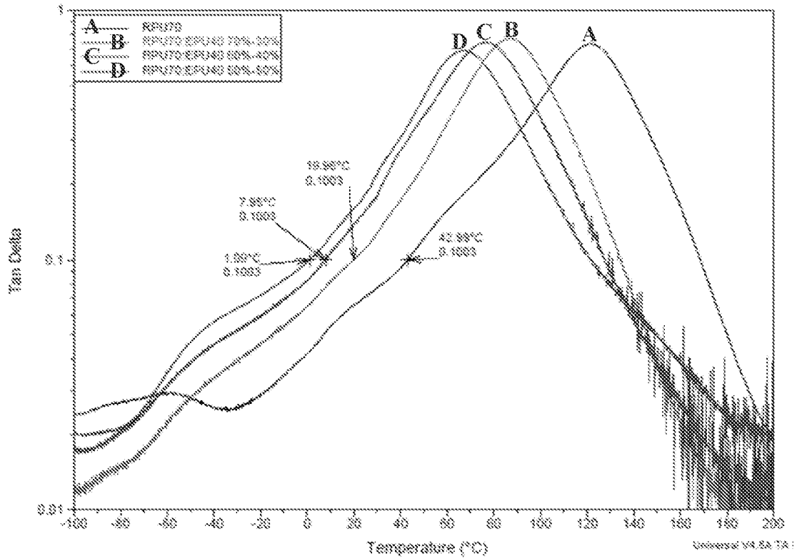
Figure 10: RPU70 + EPU40 Temperature where TanD = 0.1
