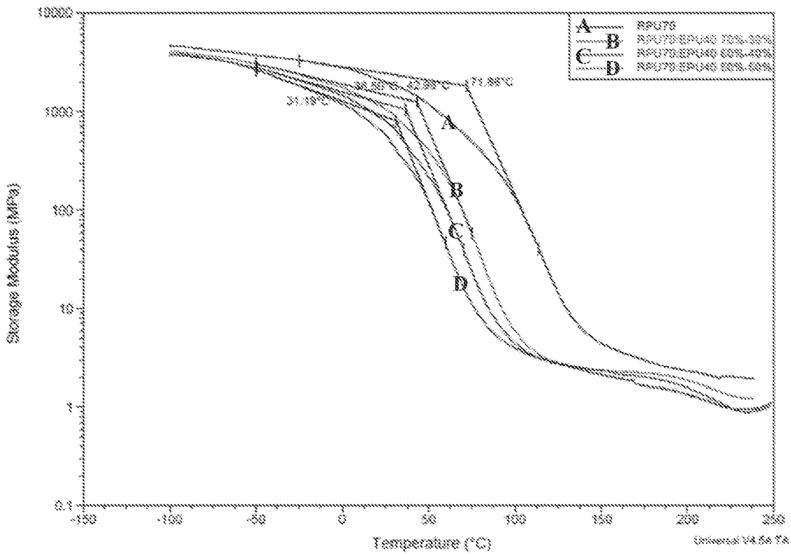
Figure 6: RPU70 + EPU40 Storage Modulus
