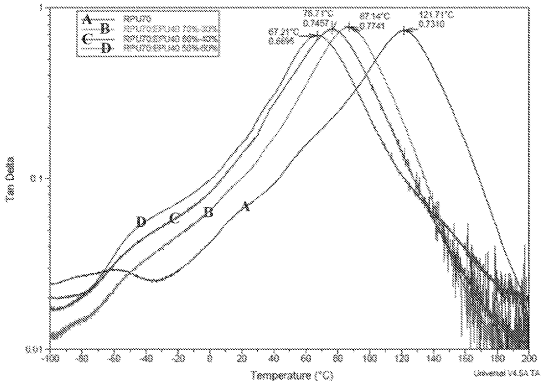
Figure 9: RPU70 + EPU40 TanD
