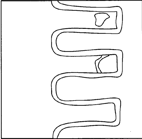
Field 3, 0.24 \mu\text{m} x 1.13 \mu\text{m} , AR = 4.7
