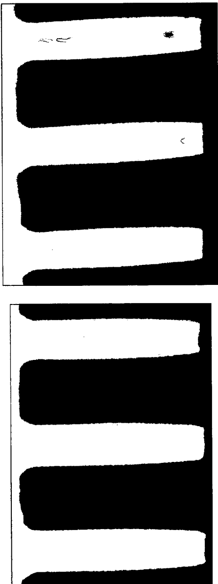
Reverse pulse matrix: Impact of t_c/t_a ratio
