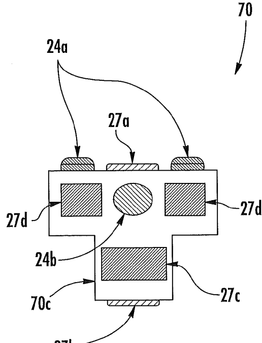
FACING EARBUD FIG. 12B
