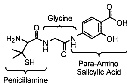
Structure of Heterodimeric Compound 1
