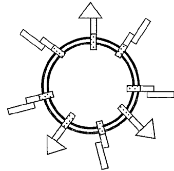
Combination of WT and Modified
