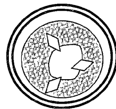
Combination of Modification and Different Species
