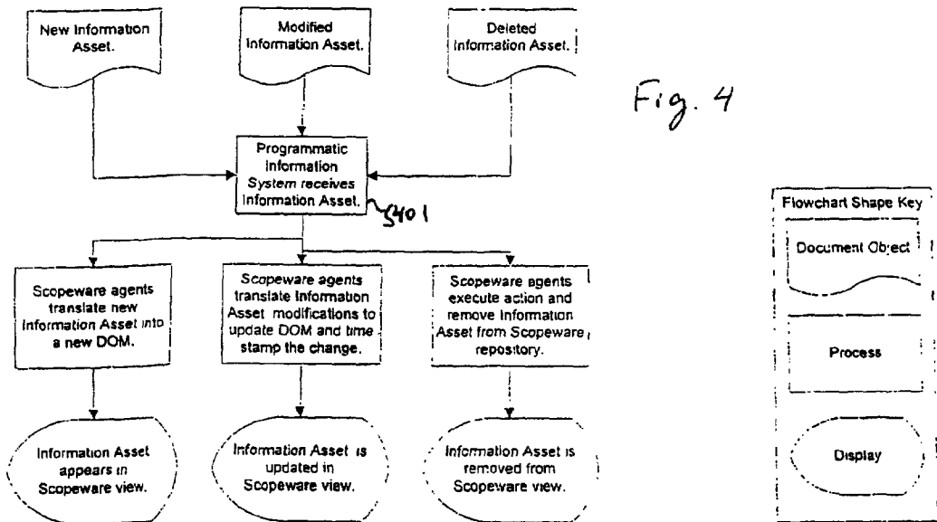
Information Assets in a Programmatic Information System
