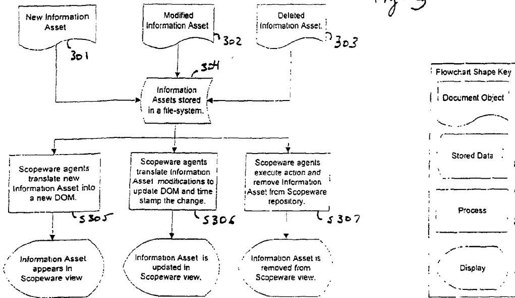
Information Assets in a File-System
