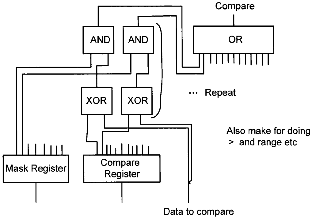
Mask and Compare Circuit
