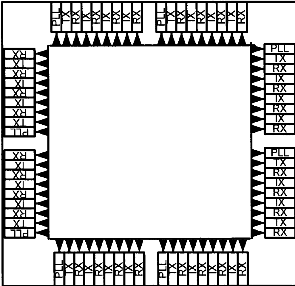
Proposed Chip 32 Channel Programmable Multi-Protocol Switch Element
