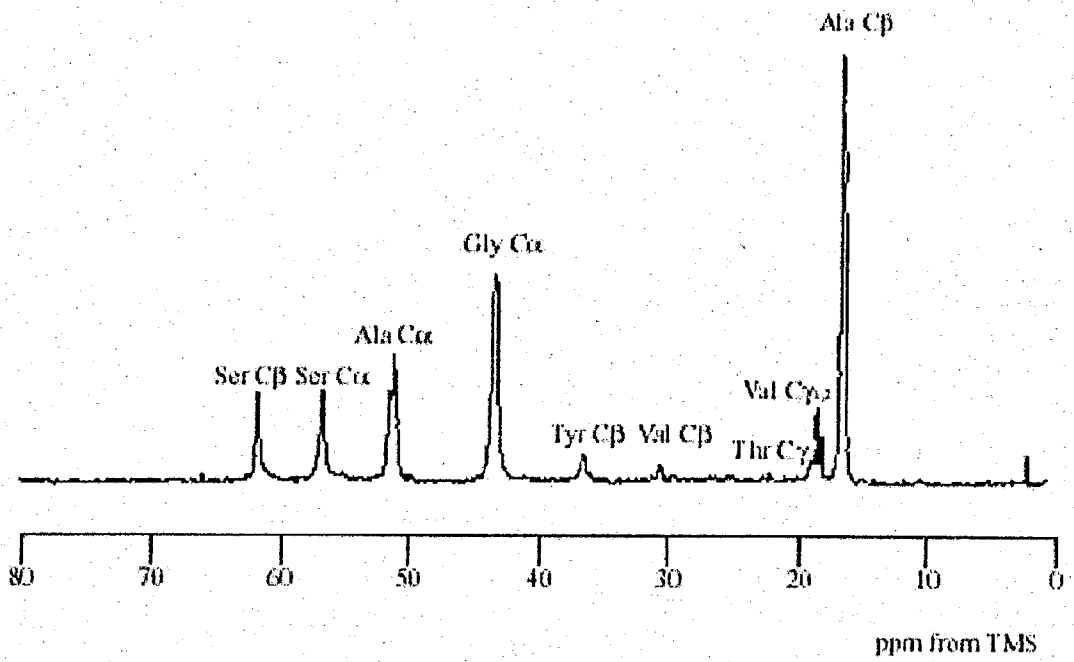
A C\alpha, C\beta region soluble 13 C NMR spectrum of B.mori fibroins in HFA hydrate.
